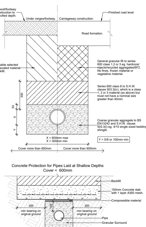
8064 - Pipe Bedding Detail Type S
