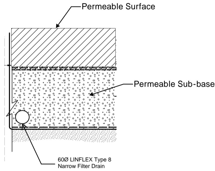
SD066 - Perforated Pipe within sub-base
