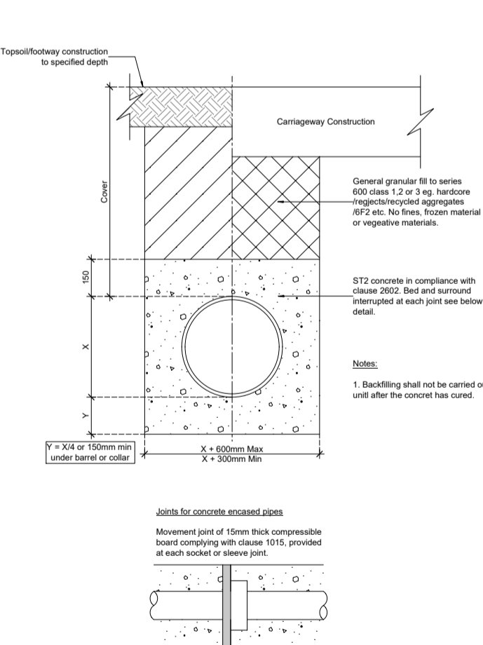
8061 - Pipe Bedding Detail Type Z
