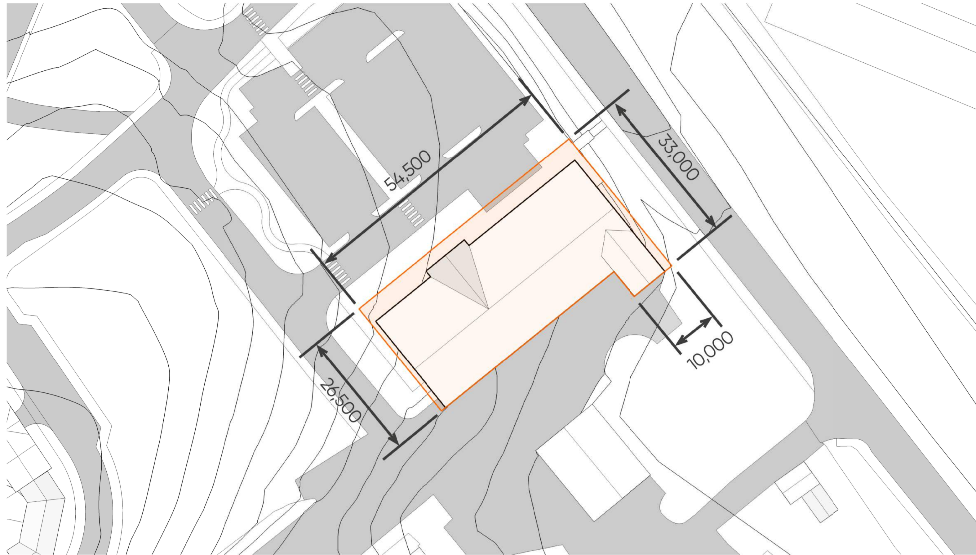
Maximum Building Extents Diagram
