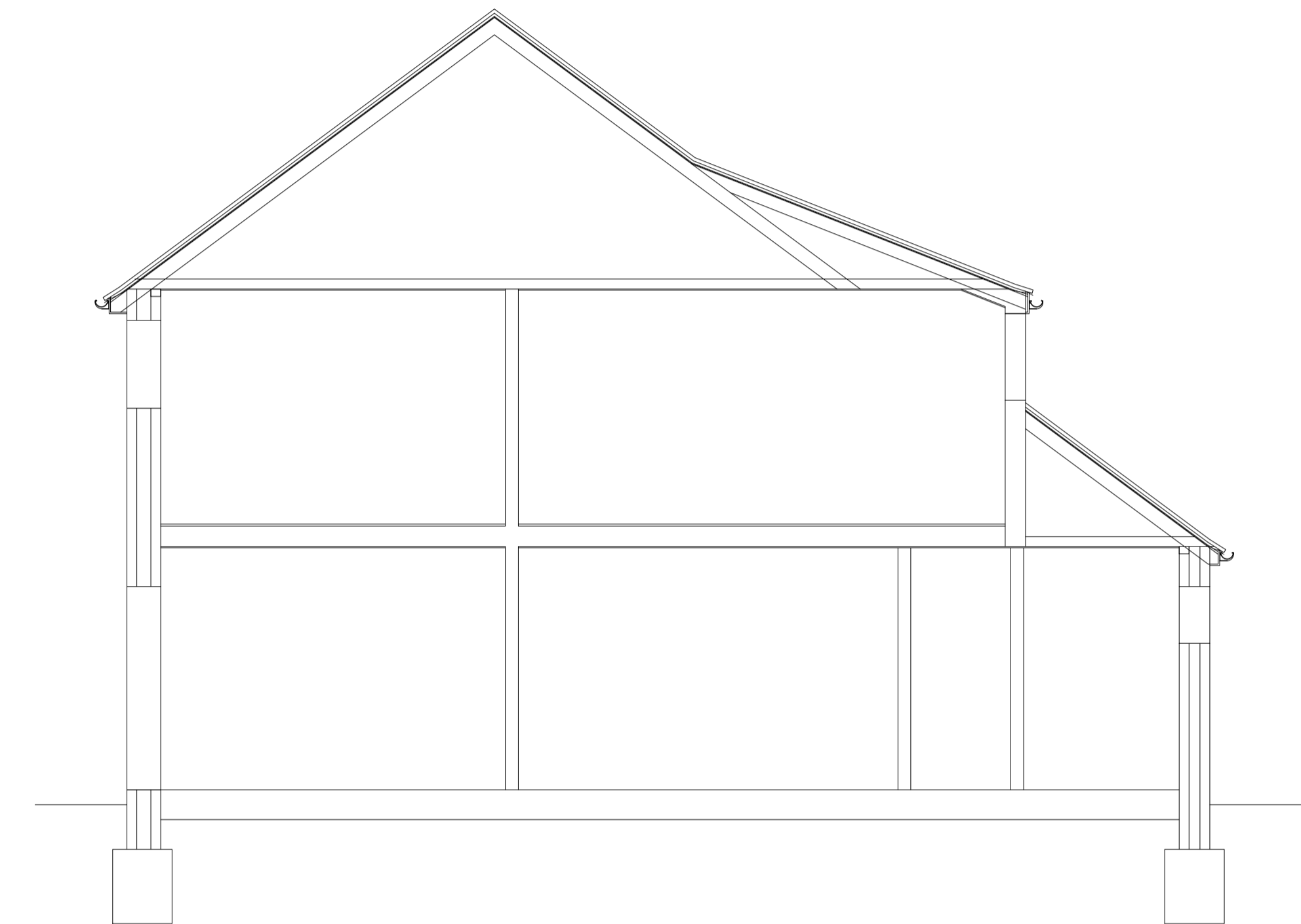
Internal Section Scale 1:50
