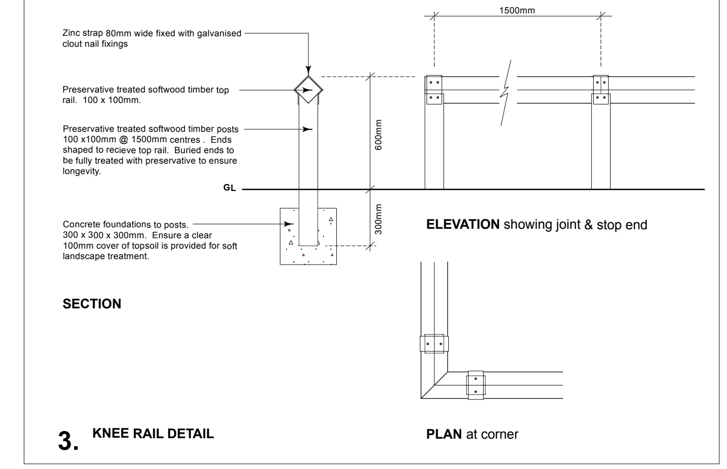
TYPICAL DETAILS Scale 1:20 @ A1
