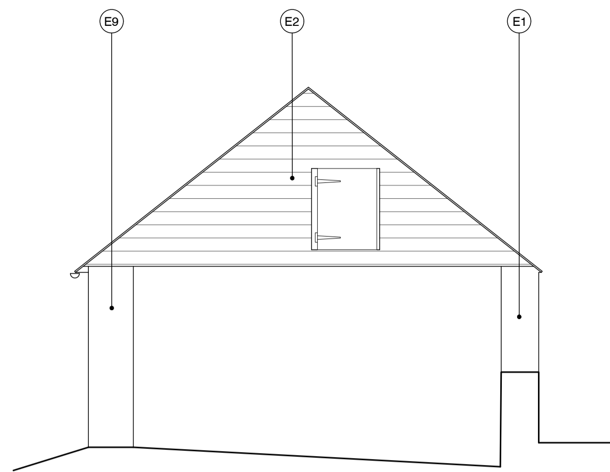
01 Elevation 3 As Existing 1:50
