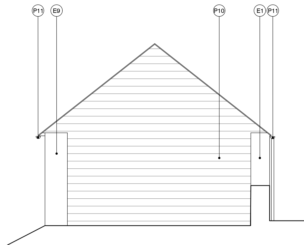
02 Elevation 3 As Proposed 1:50
