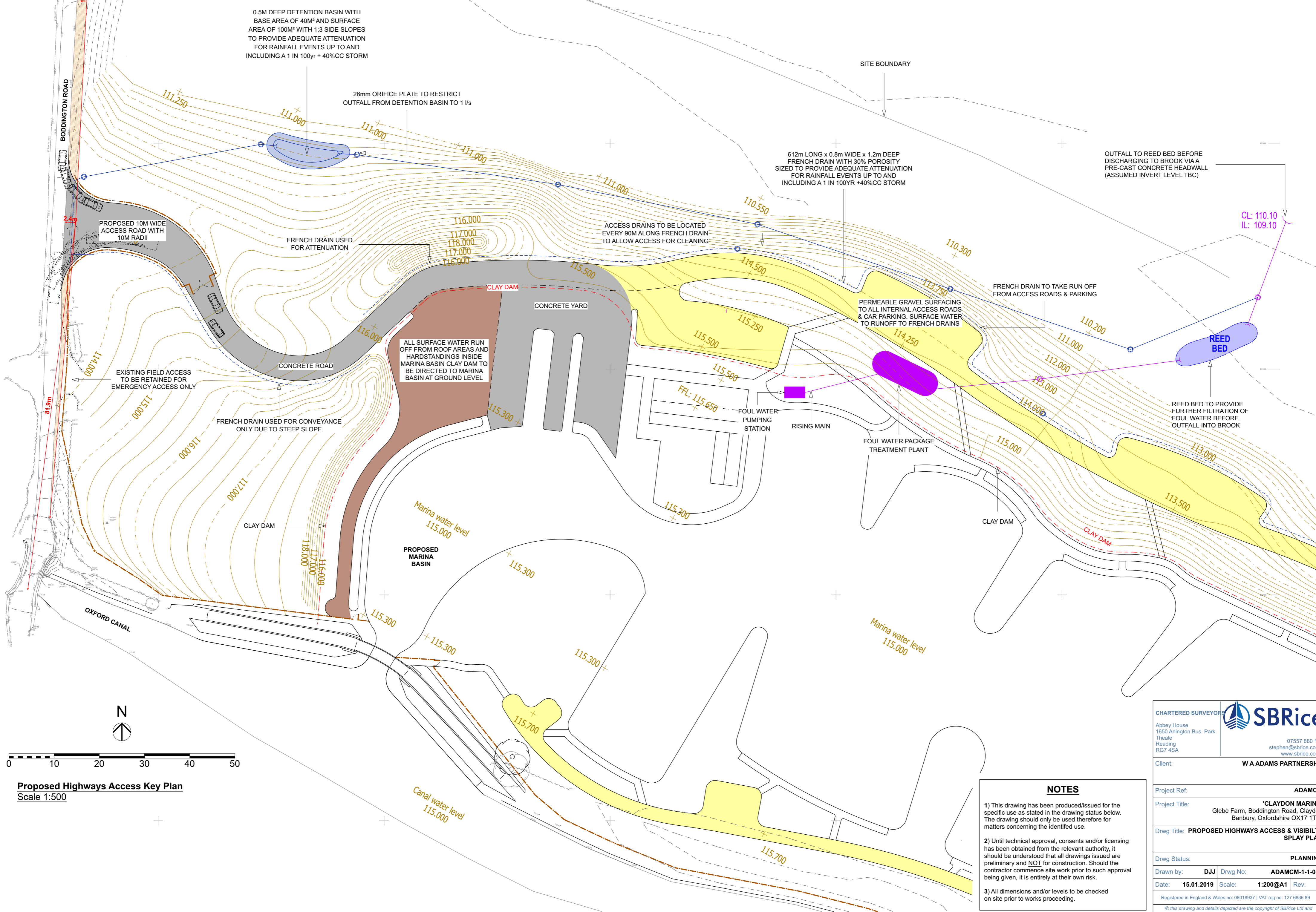
Proposed Highways Access Scale 1:200
