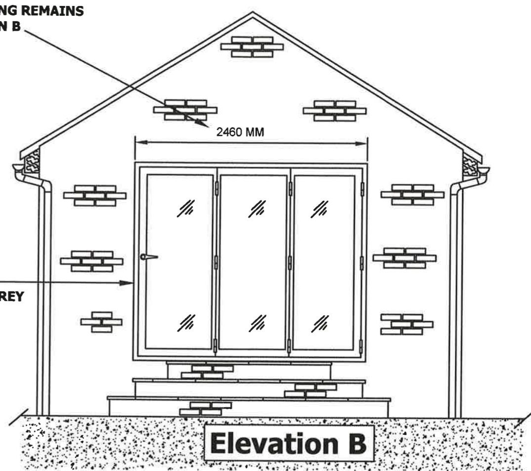
PROPOSED REAR ELEVATION OF HINGED BI-FOLDING EXTERIOR DOORS WITH THREE GLAZED SECTIONS. ALL THREE DOORS WILL FOLD TO THE RIGHT HAND SIDE OF THE APERTURE. OPTION TO OPEN SINGLE DOOR PANEL AT THE LEFT HAND END.
