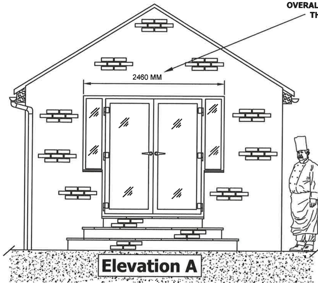
EXISTING REAR ELEVATION OF SIDE HINGED EXTERIOR DOUBLE DOORS WHICH OPEN OUTWARDS OVER THE SECTION OF THREE TIER STEPS
