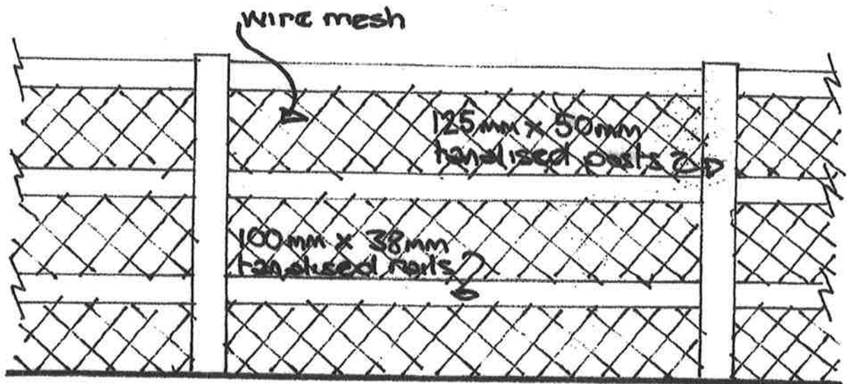
Post & rail fence 1:20
