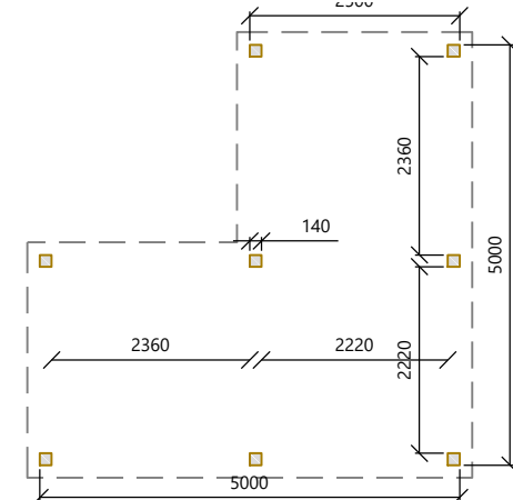
Proposed Plan Scale. 1:100
