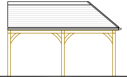
Proposed North Elevation Scale. 1:100
