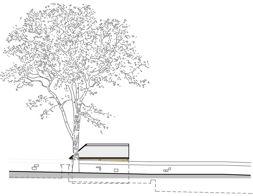
2 - 2 Proposed West Elevation / Section Scale. 1:200
