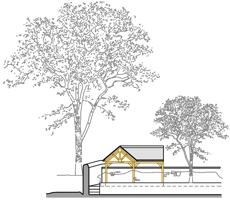
3 - 3 Proposed South Elevation / Section Scale. 1:200
