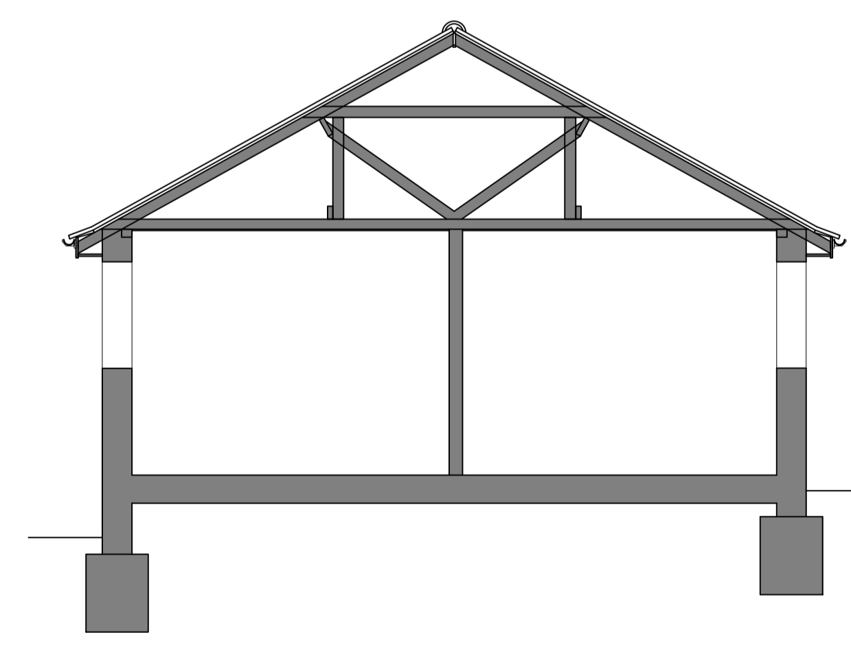
Typical Section Scale 1:50 0.0m 1.0m 2.0m 3.0m 4.0m 5.0m Roof Make Up 47x97mm ceiling joists 50x100mm rafters 50x125mm binders 50x180mm purlins 50x105 collars & struts
