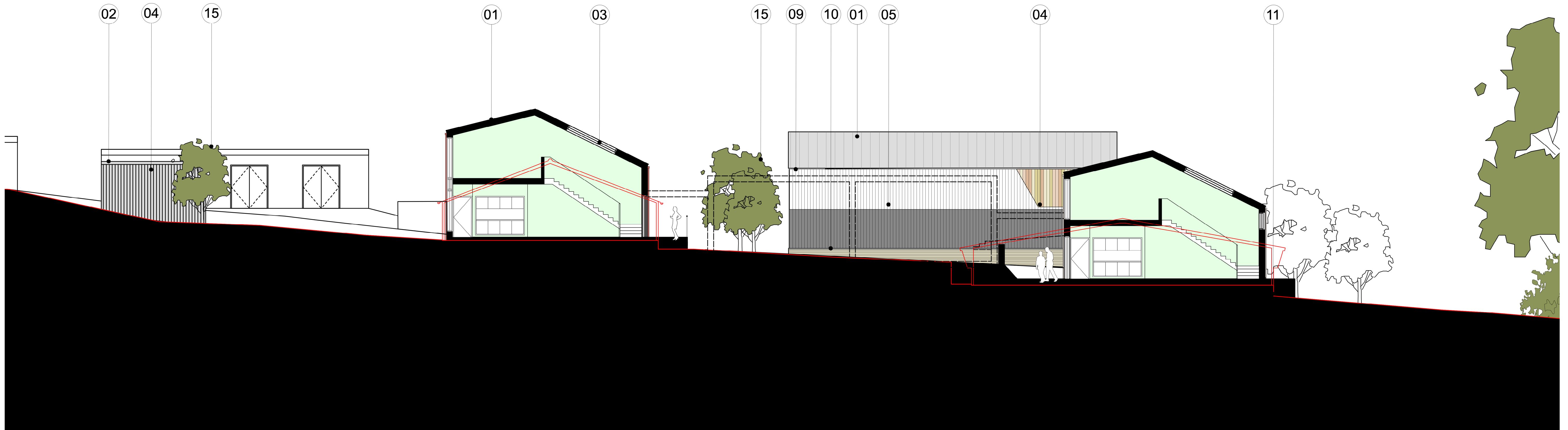
2 Proposed Section C-C Scale: 1:100
