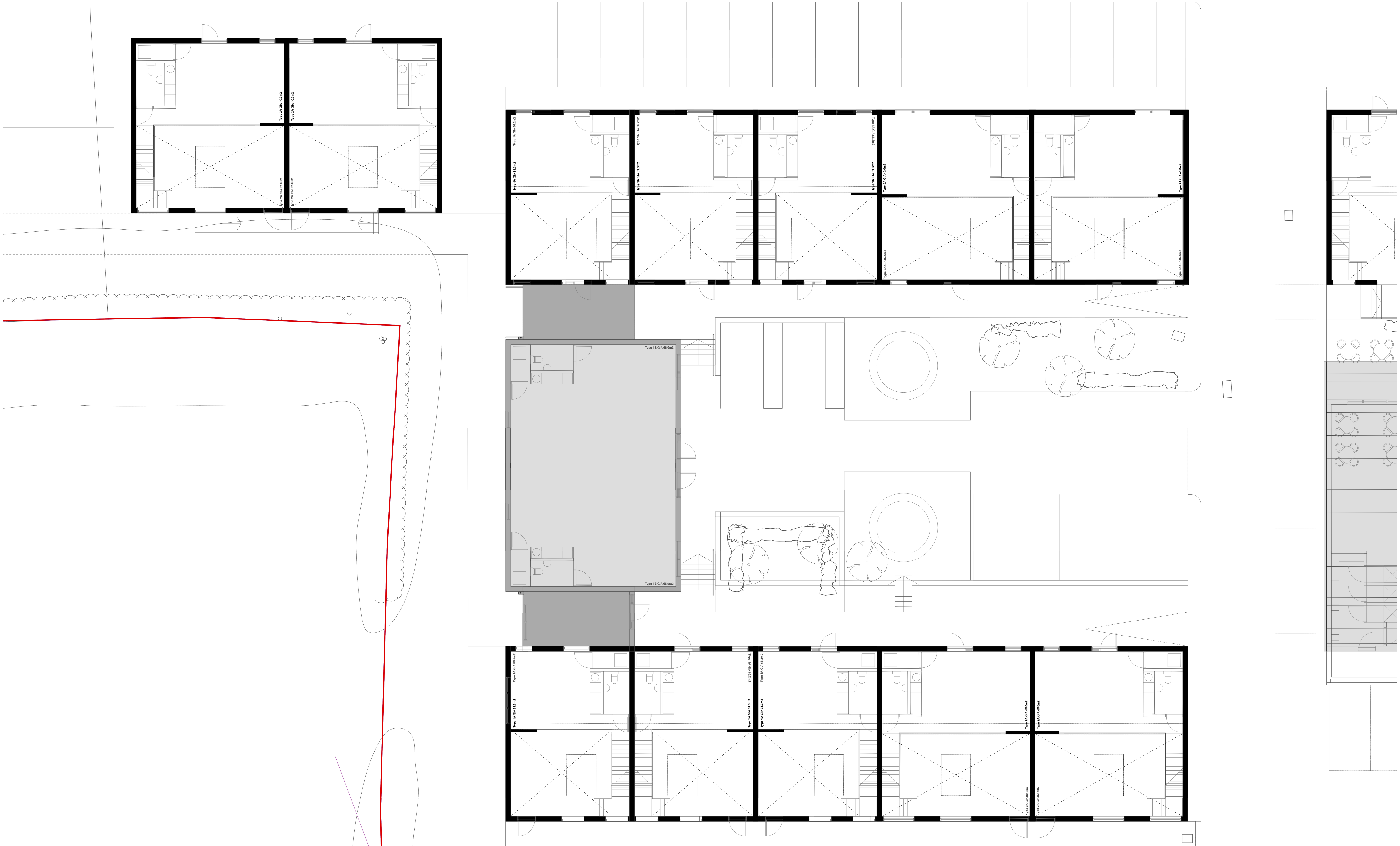
1 Proposed Building Plan 1 (South Site Area) Scale: 1:100
