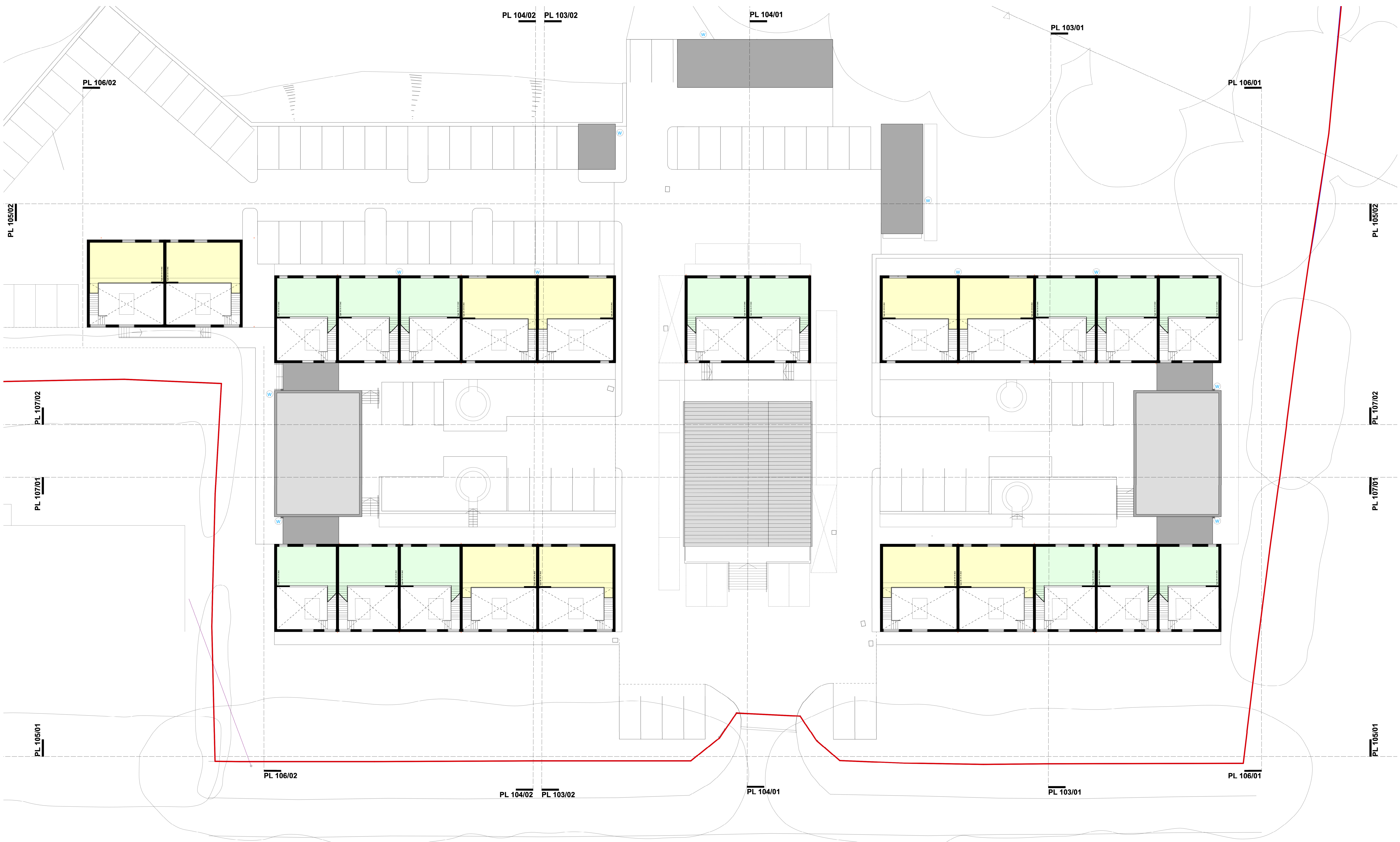
1 Proposed Site Plan - Mezzanine Floor Scale: 1:200
