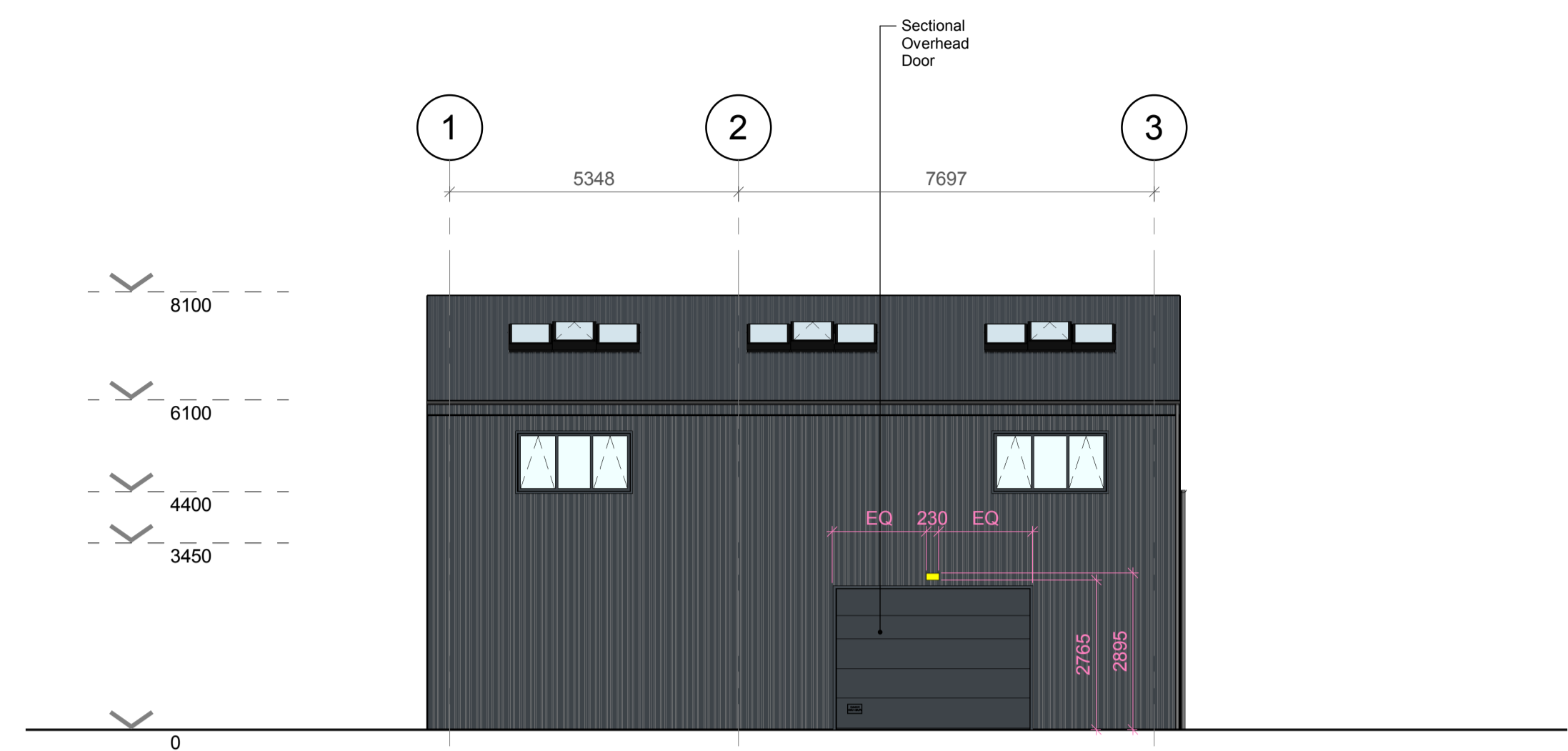
2. NW Elevation 1 : 100
