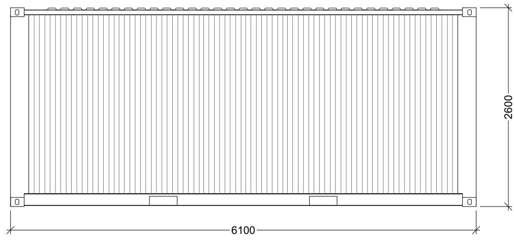
REAR VIEW
