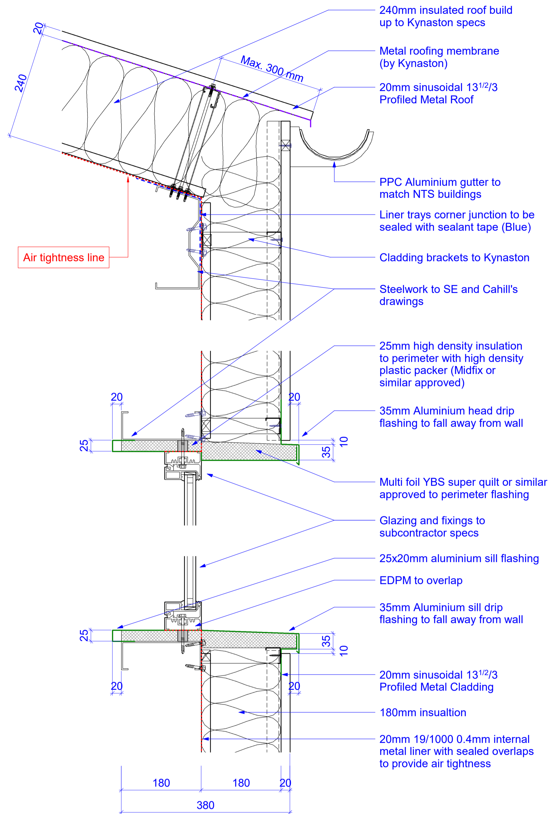
Metal Cladding - Window Head & Sill Flashing 1 : 5
