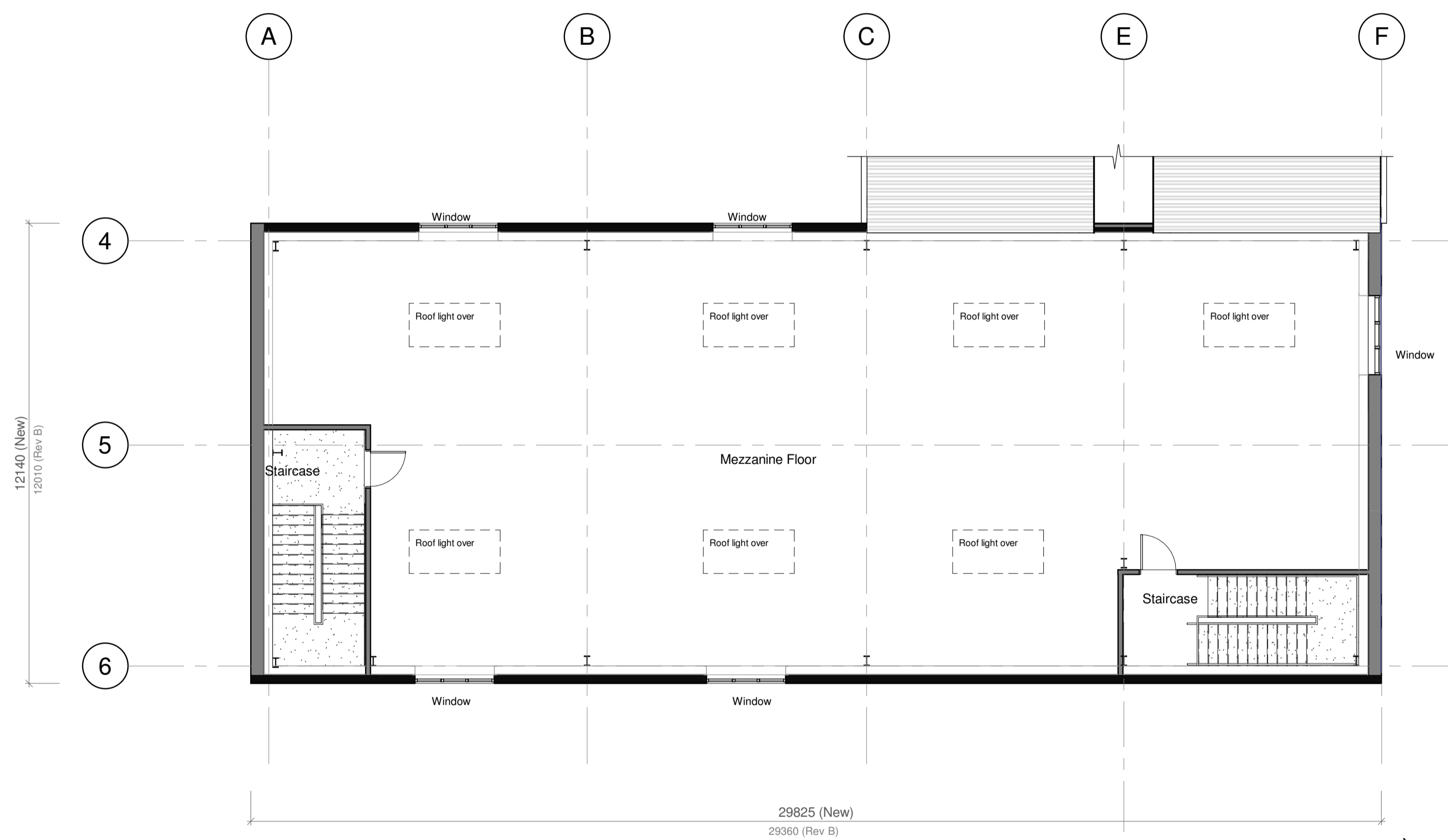
Mezzanine Floor 1 : 100
