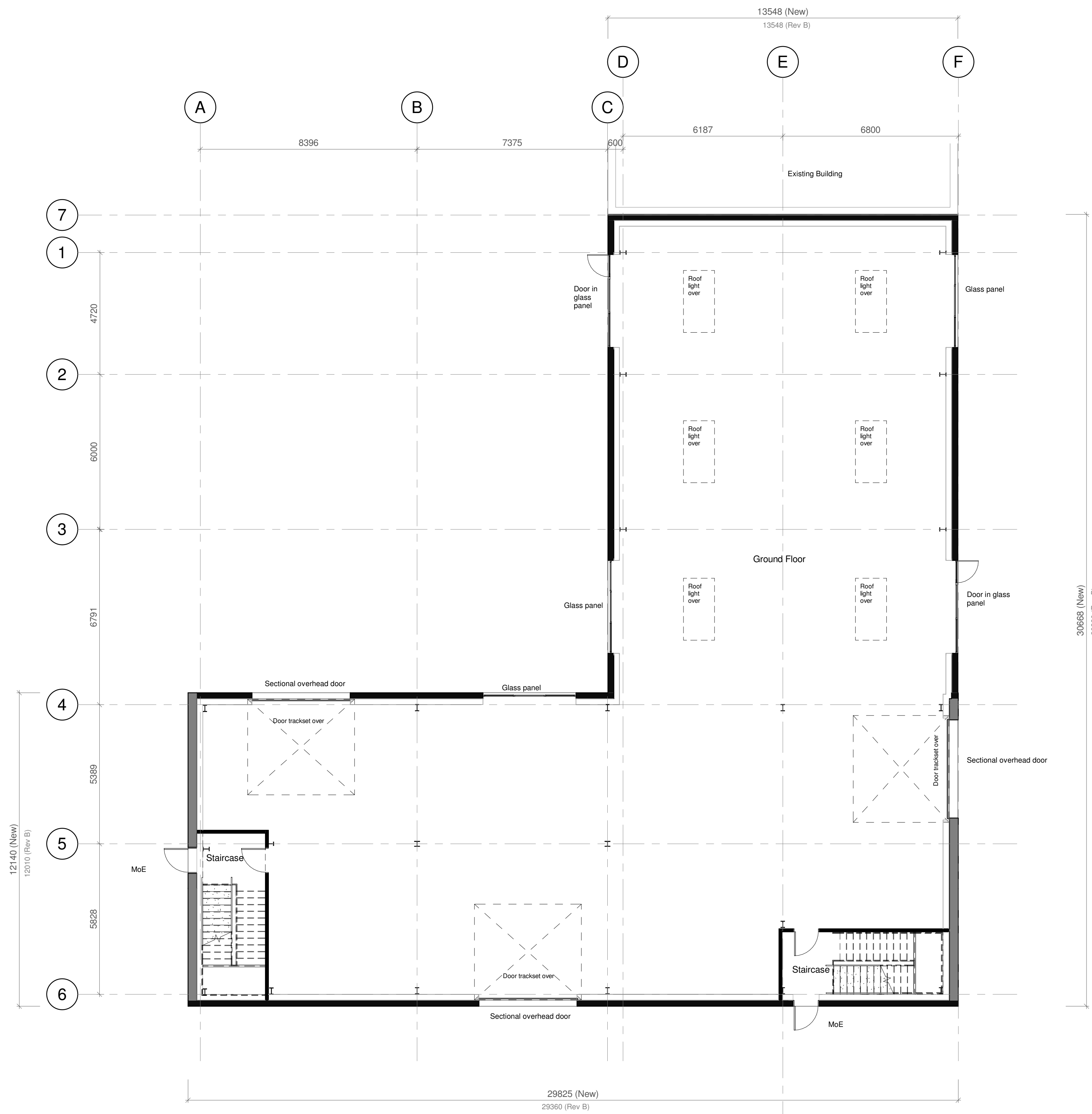
Ground Floor Plan 1 : 100
