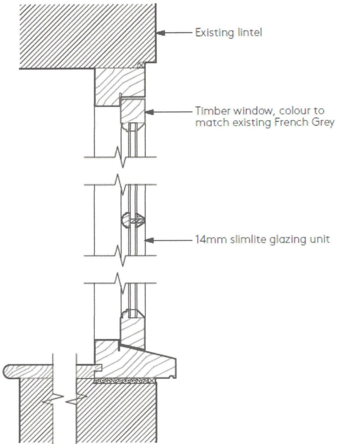
Typical Window Head, Cill & Glazing Bar Detail Scale: 1:5
