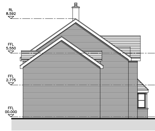
Left Elevation
