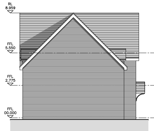
Left Elevation
