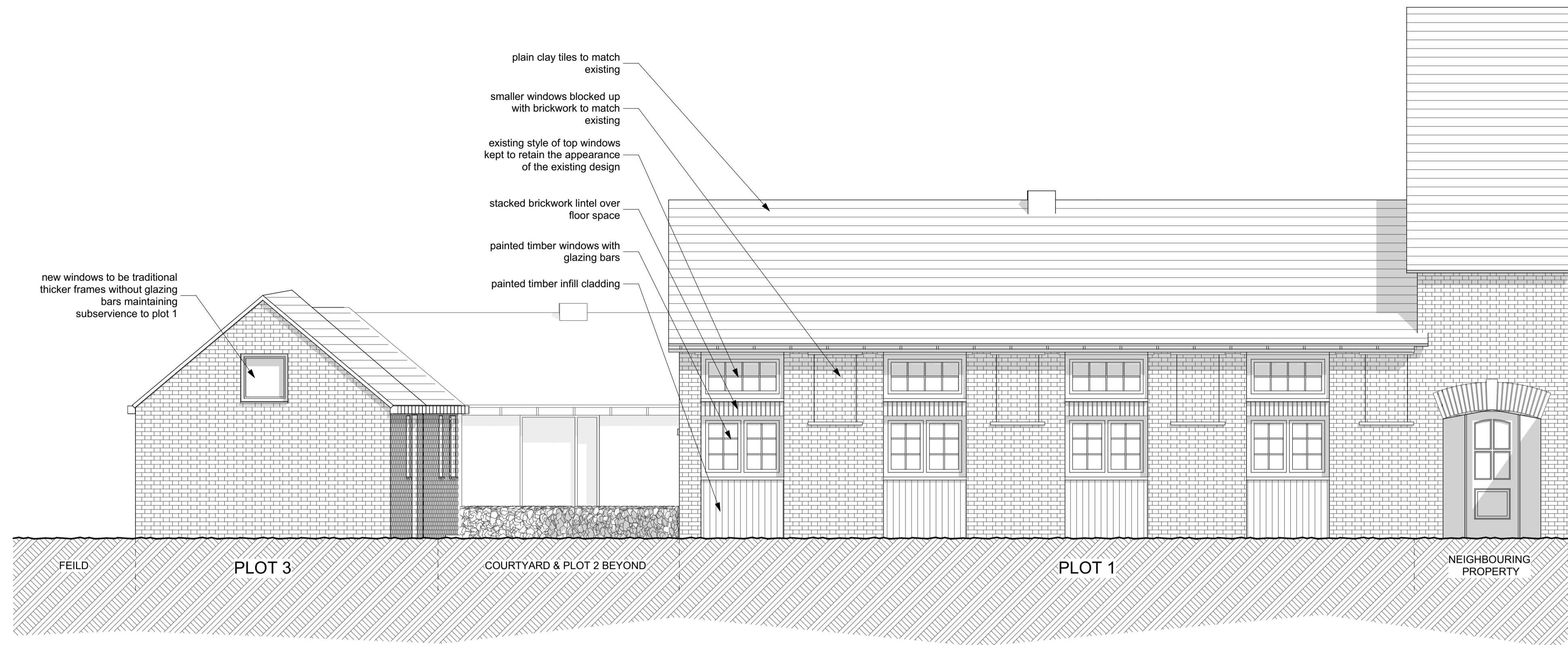
A-A PROPOSED ELEVATIONS 211 Scale: 1:50 @ A1 / 1:100 @ A3
