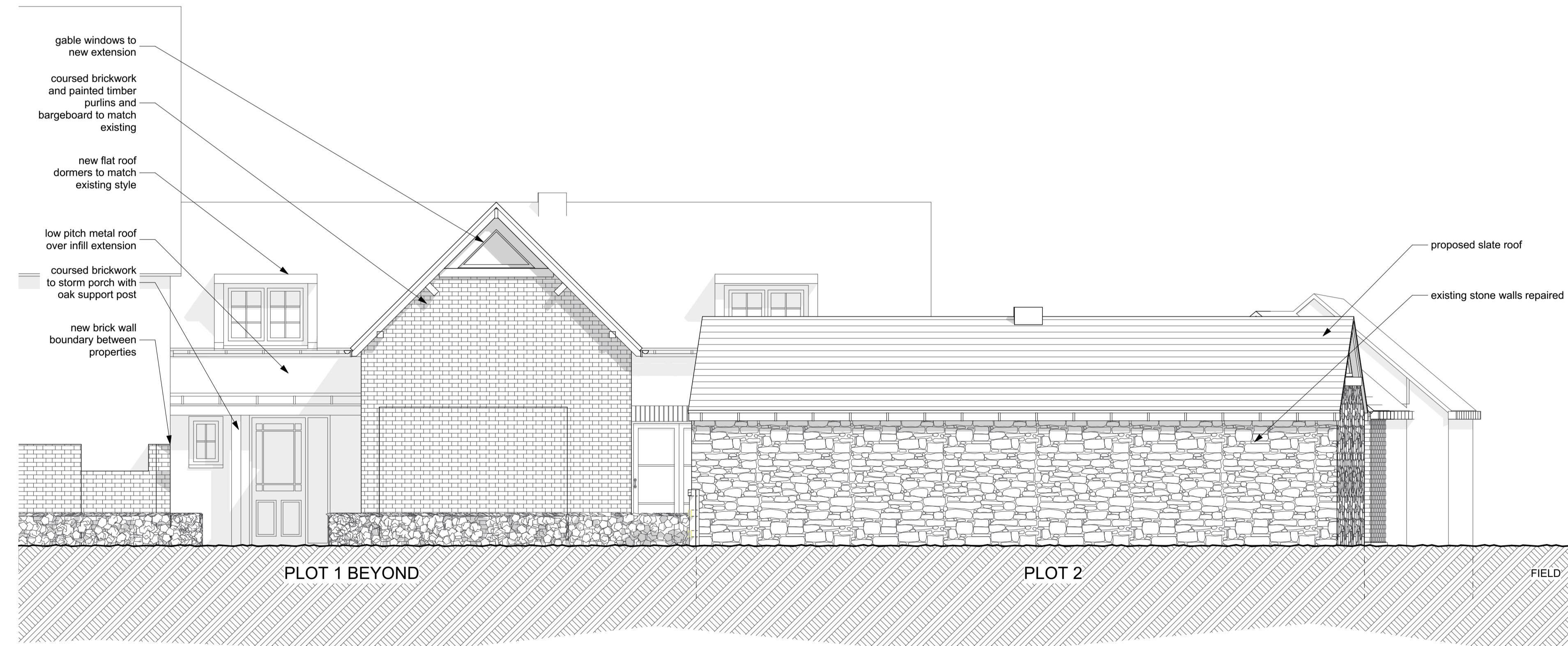
B-B PROPOSED ELEVATIONS 211 Scale: 1:50 @ A1 / 1:100 @ A3
