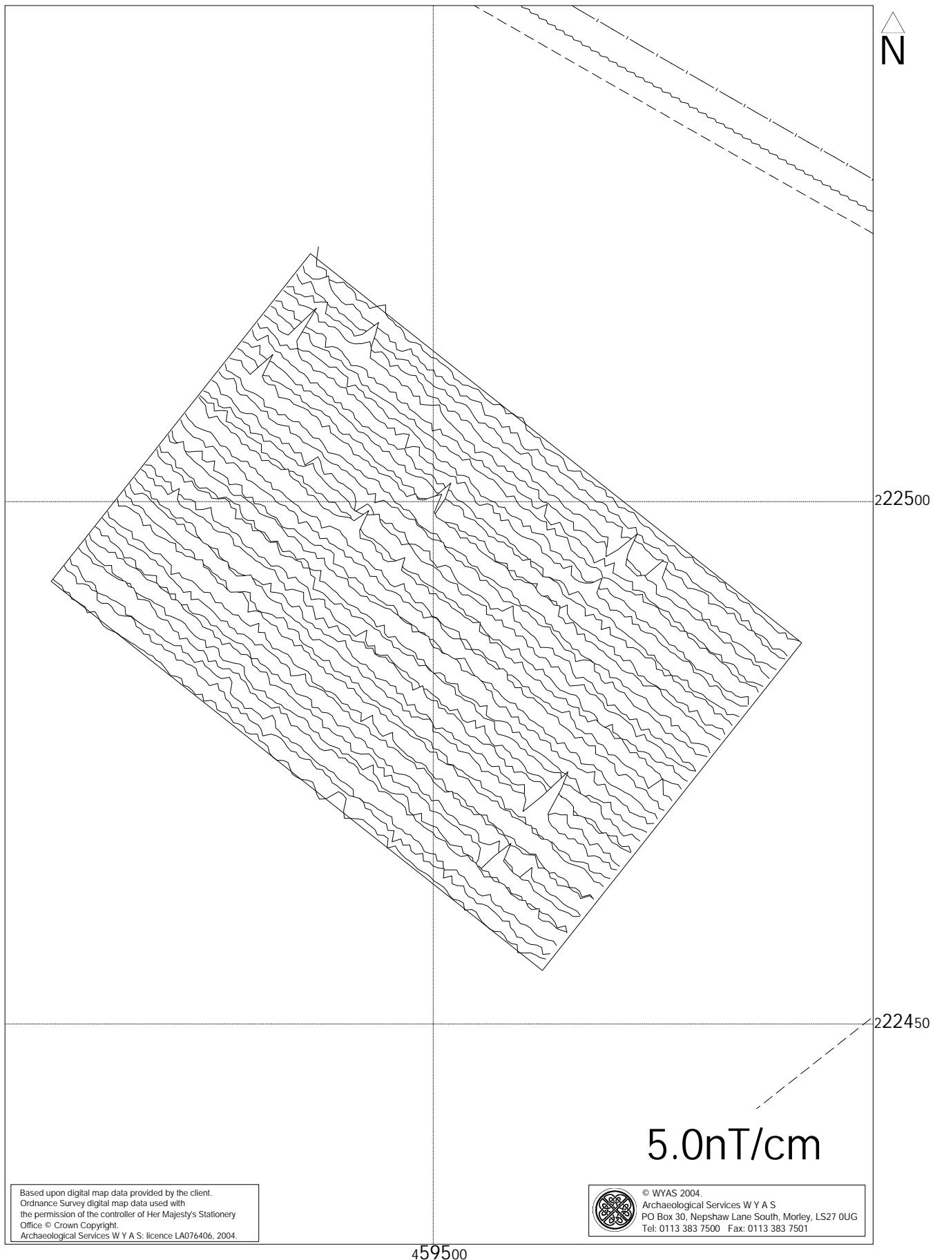
Fig. 5. XY trace plot of gradiometer data; Block 1
