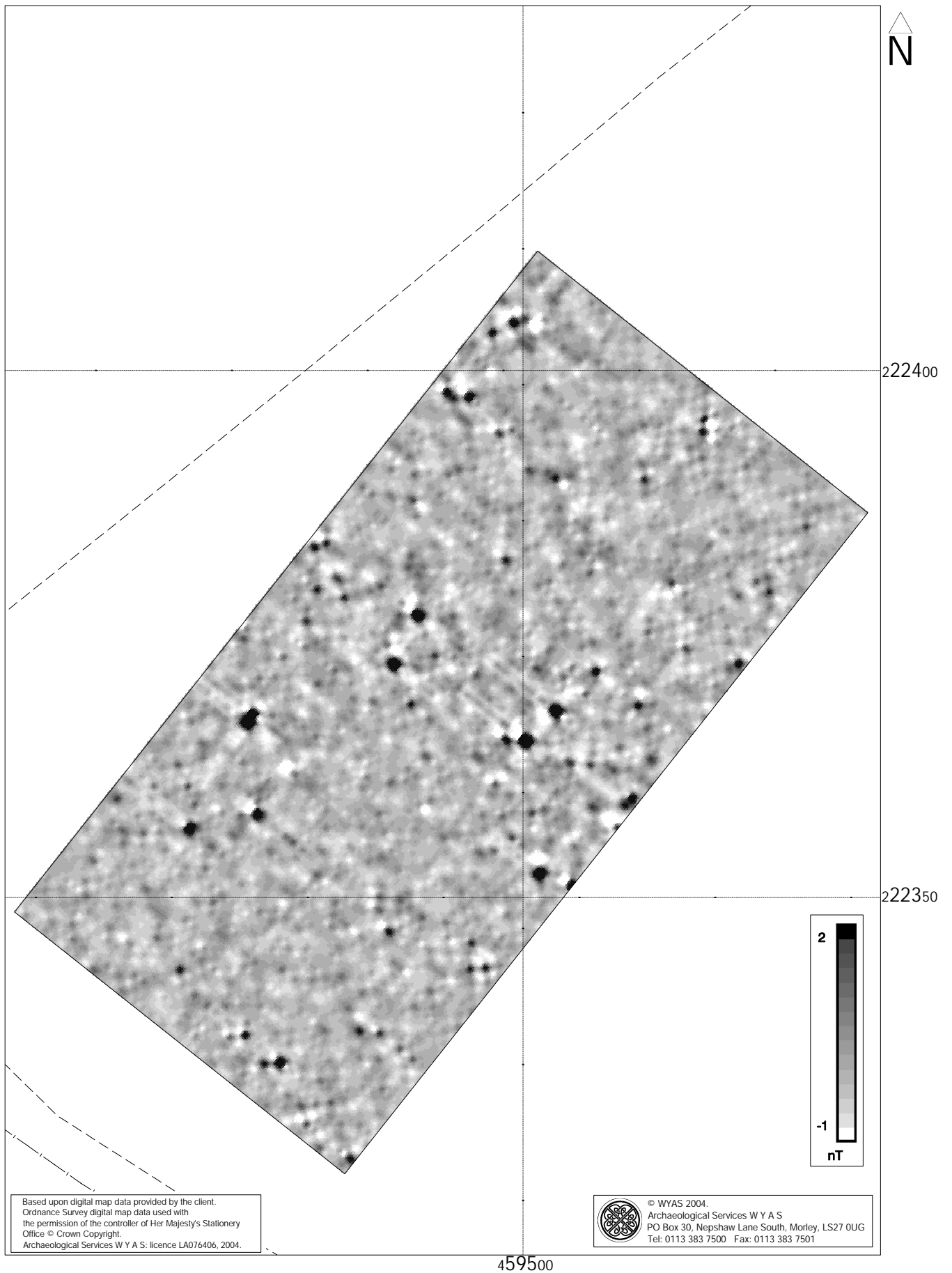
Fig. 12. Greyscale plot of gradiometer data; Block 4
