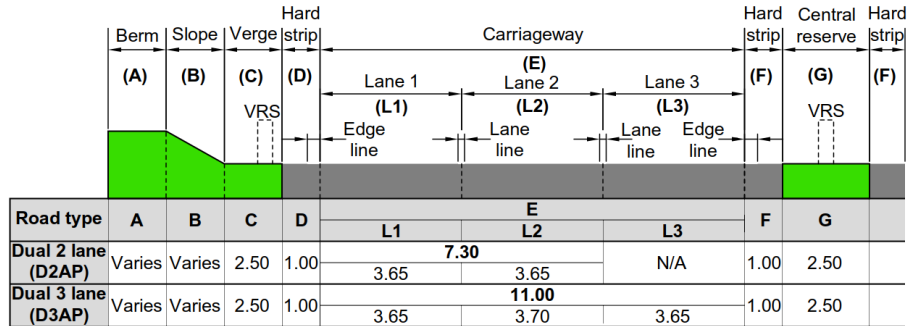
Figure 2.1.1N1e Dimensions of cross-section components for rural all-purpose roads mainline
