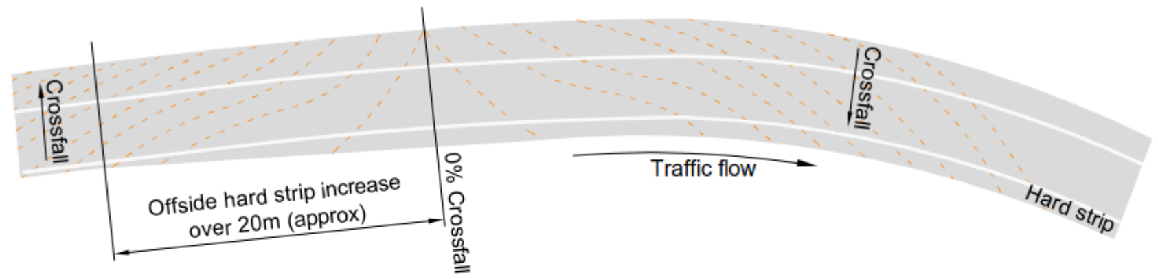
Figure 2.30.1 Offside hard strip width changes Offside hard strip increase
