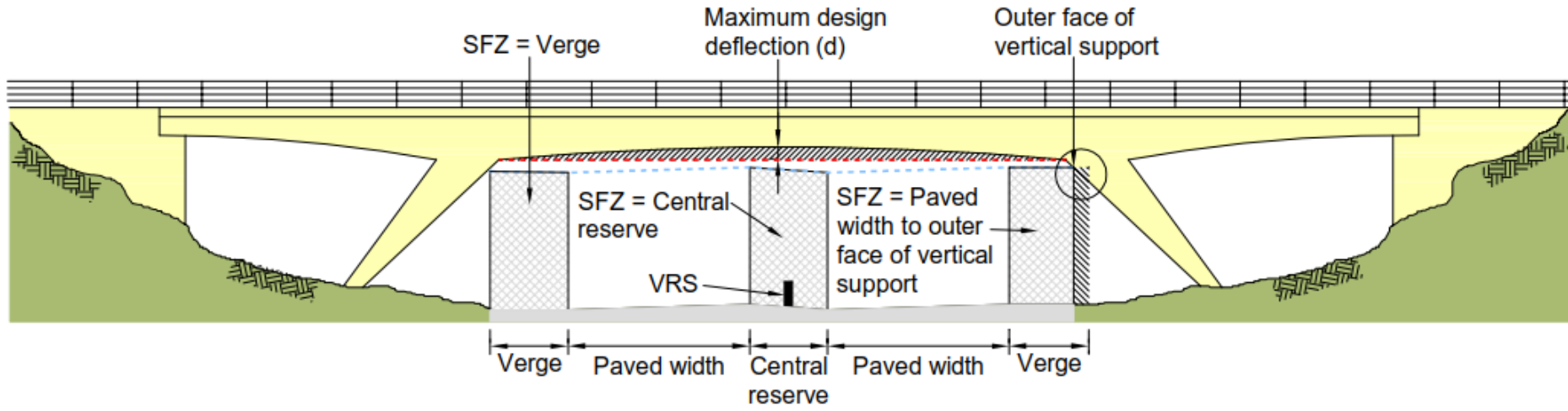
Figure 4.6N1 Minimum width of the SFZ
