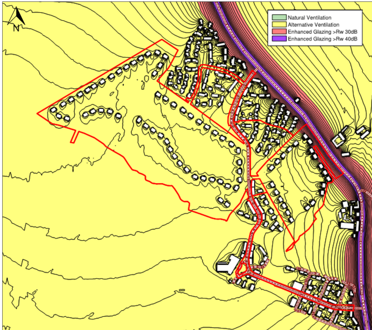
Figure 8.7: Indicative Glazing and Ventilation Strategy – Bedrooms (Grid Height 4.0m)
