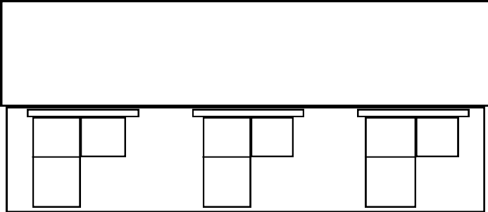
SOUTHERN ELEVATION
