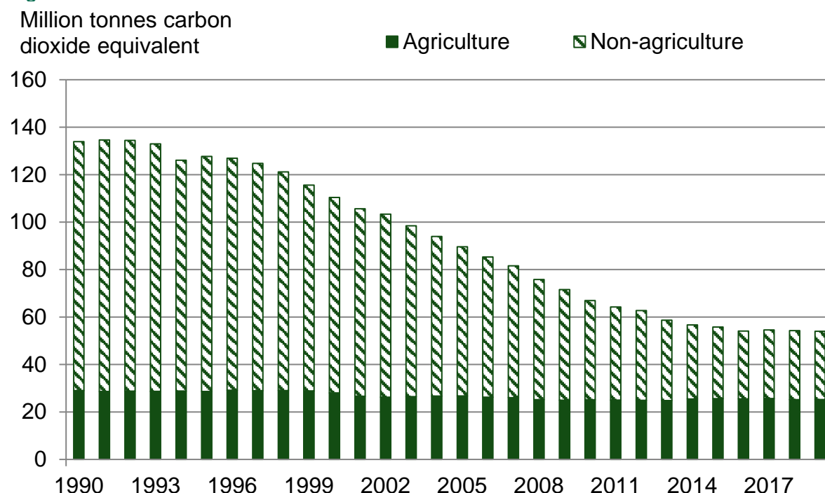
Figure 11.10 Methane emissions
