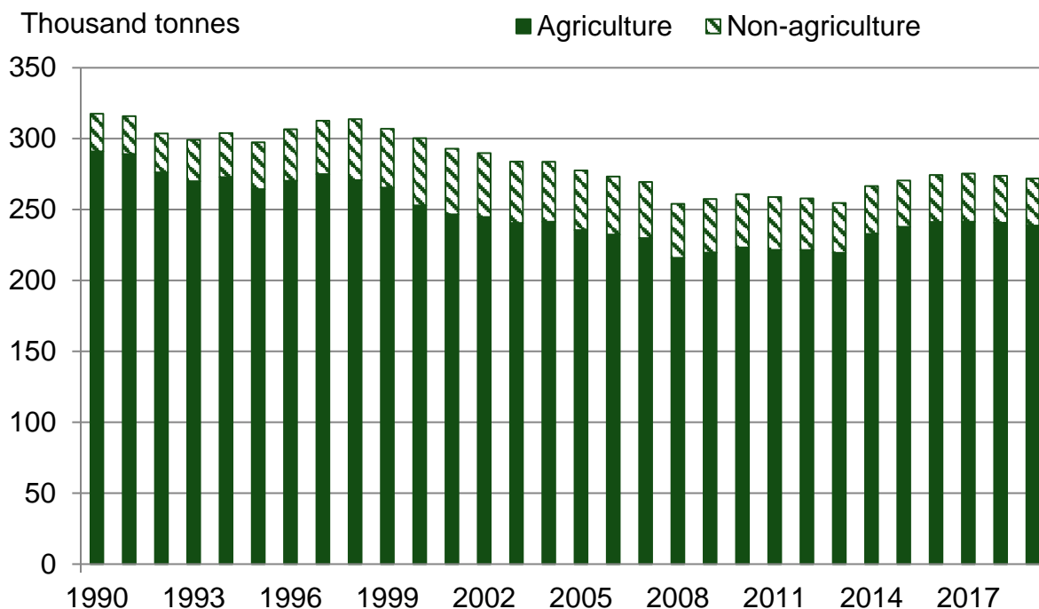
Figure 11.11 Ammonia Emissions
