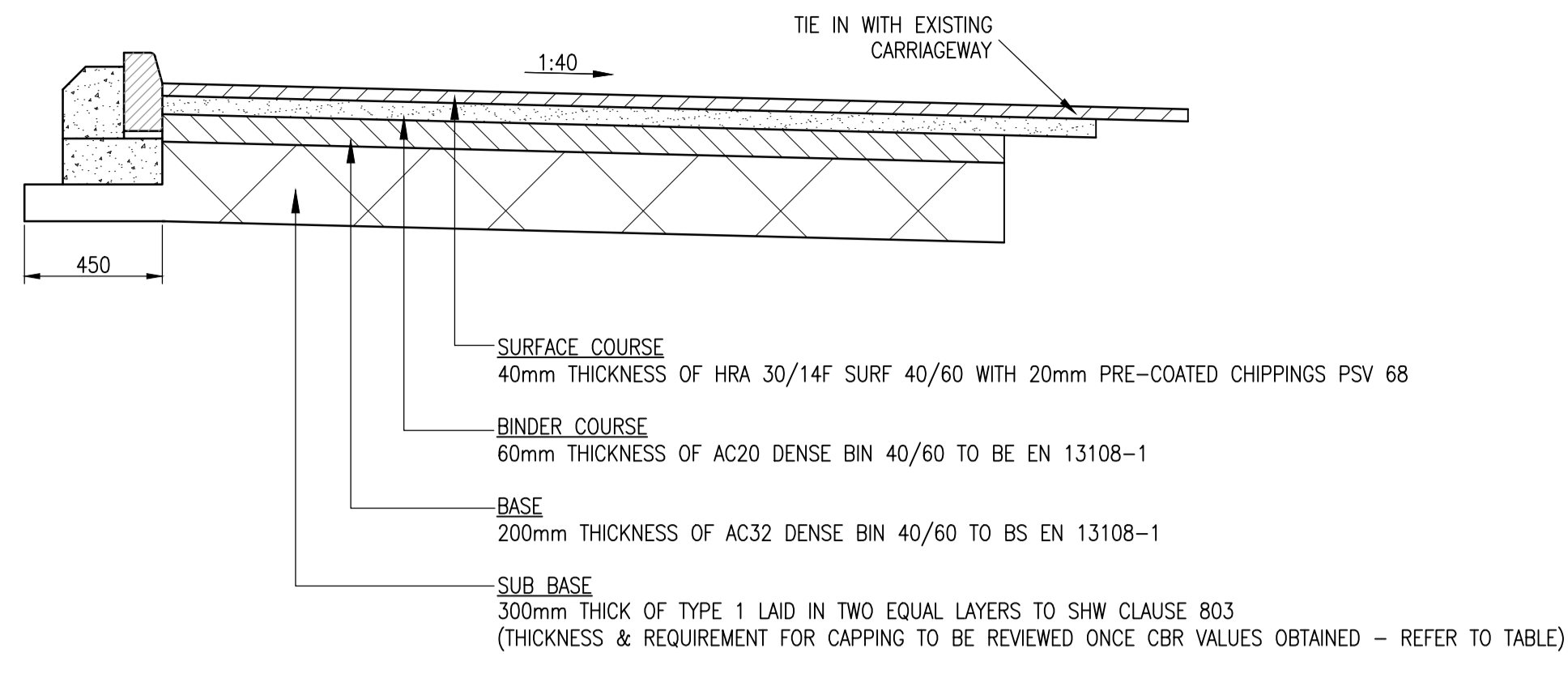
PASSING BAY CONSTRUCTION CROSS SECTION SCALE 1:20
