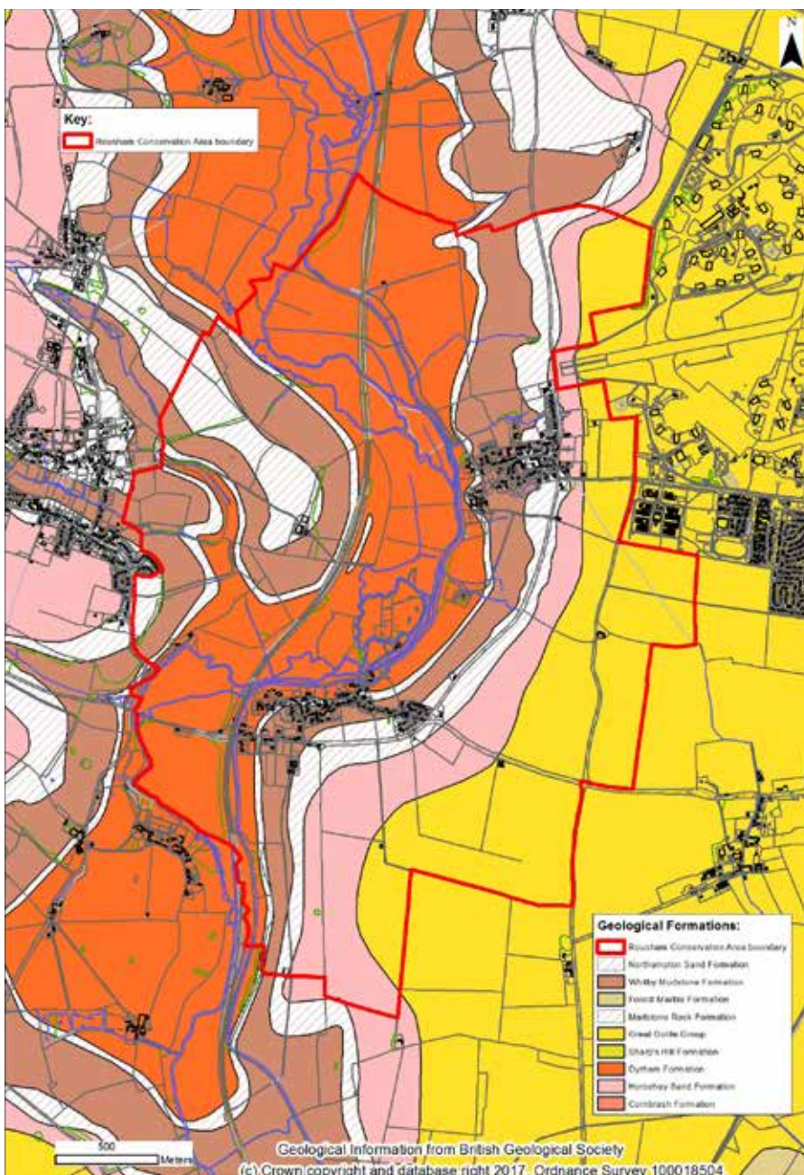
Figure 6. Geological map
