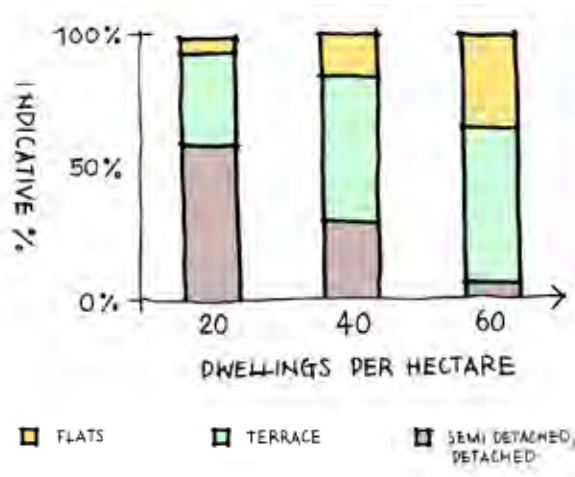
Figure 4.13 Indicative split of house typologies at different densities
