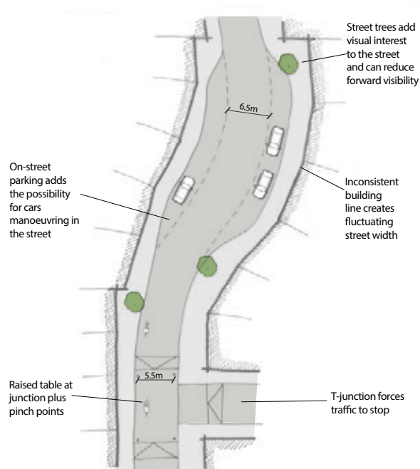
Figure 5.10 Traffic calming measures along a street
