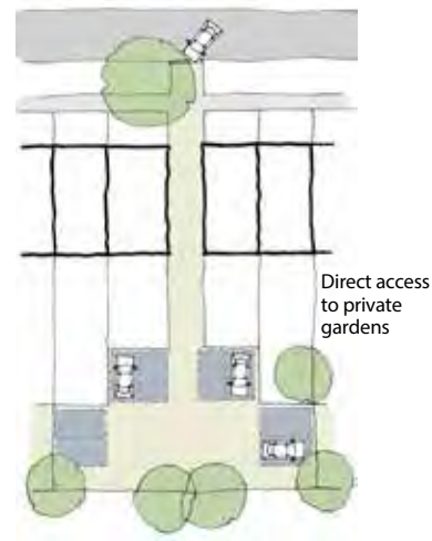
Figure 5.13 Example of private rear parking court
