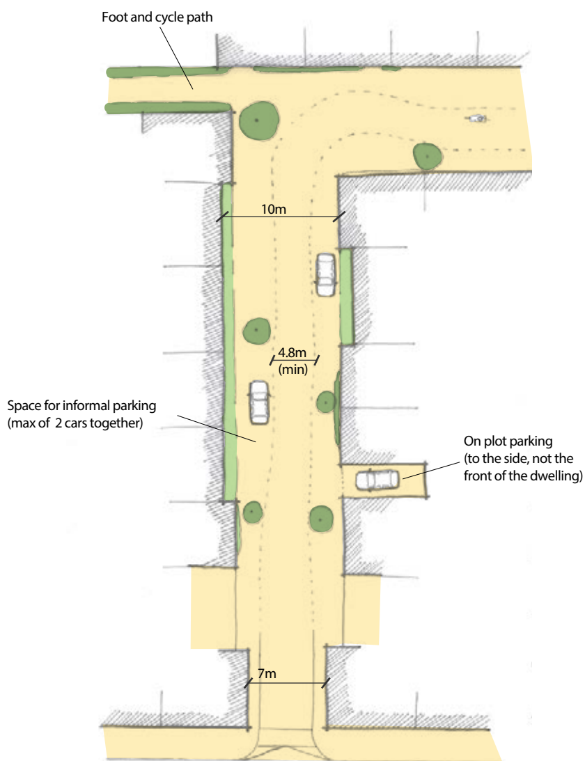
Figure 5.6 Indicative layout - Shared surface street
