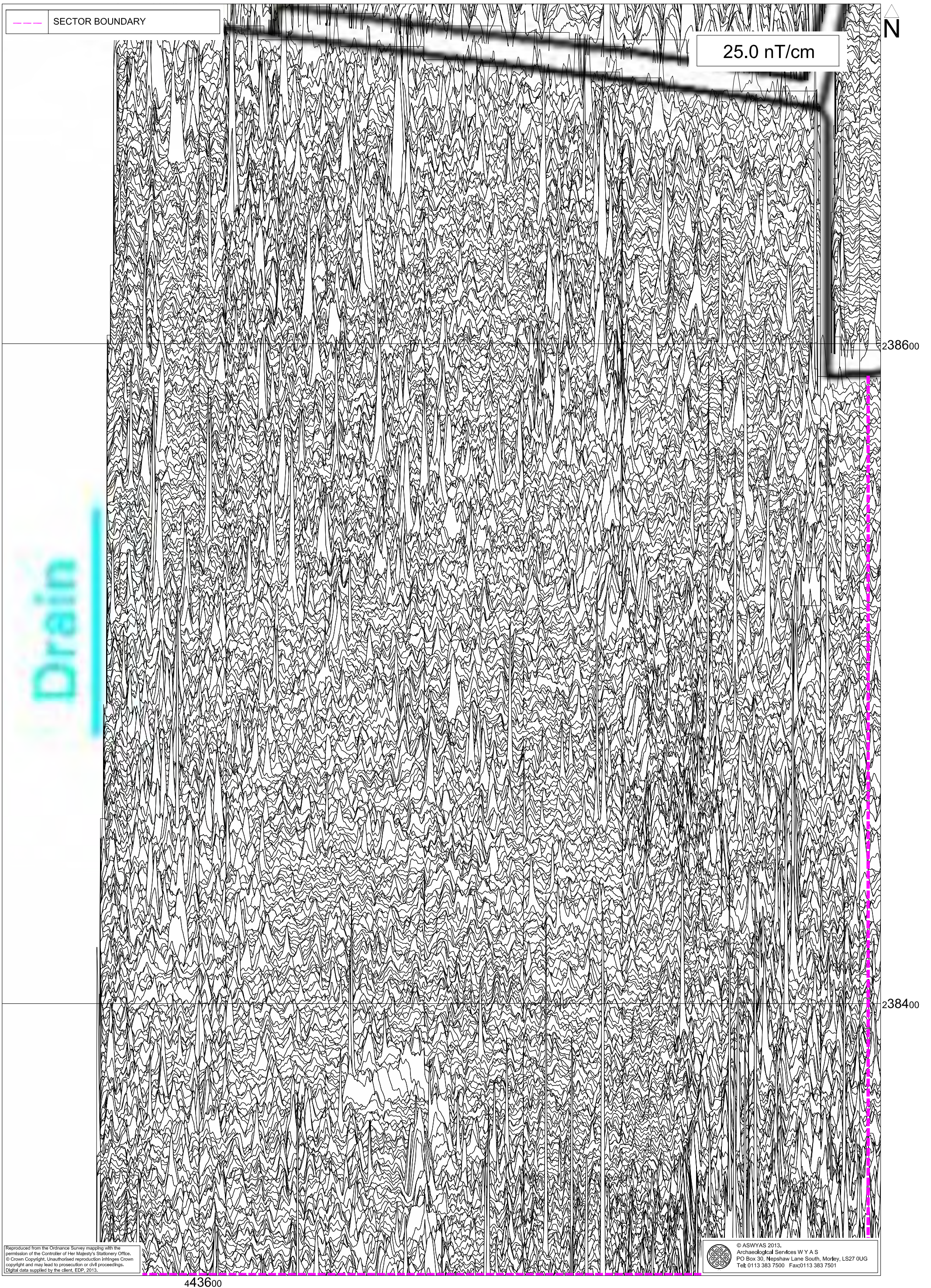
Fig. 24. XY trace plot of minimally processed magnetometer data; Field 6, Sector 3 (1:1000 @ A3)
