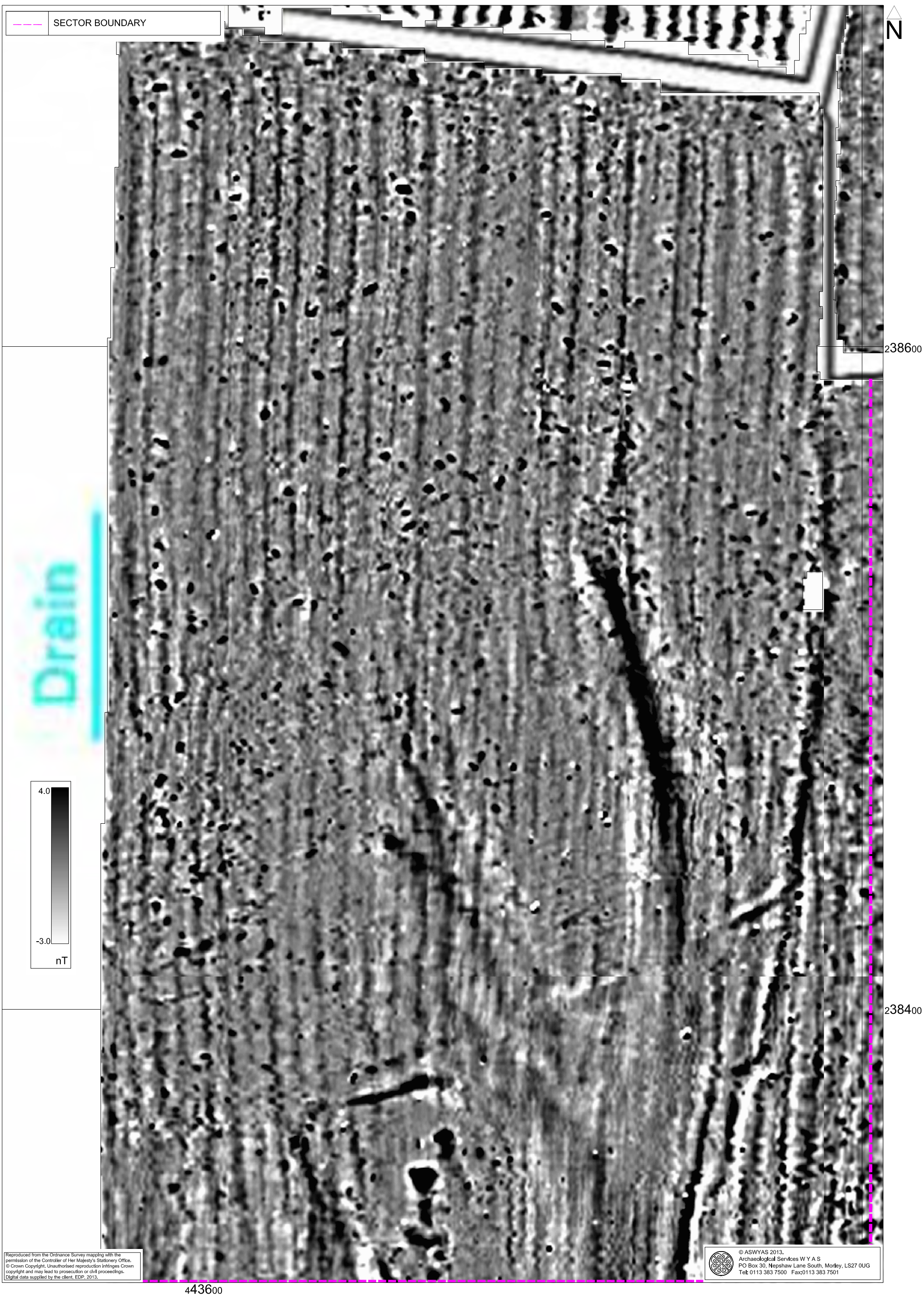
Fig. 23. Processed greyscale magnetometer data; Field 6, Sector 3 (1:1000 @ A3)
