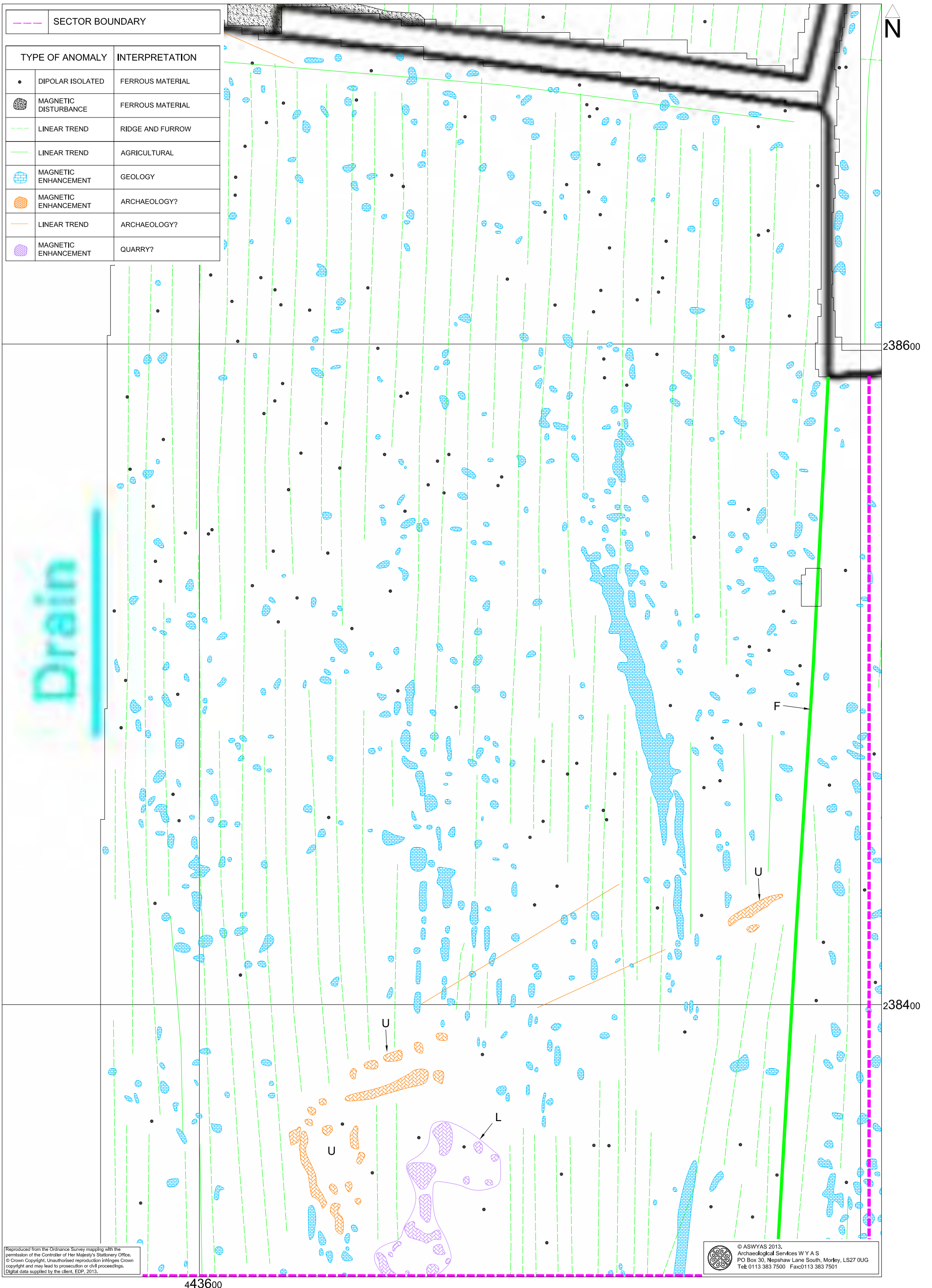
Fig. 25. Interpretation of magnetometer data; Field 6, Sector 3 (1:1000 @ A3)
