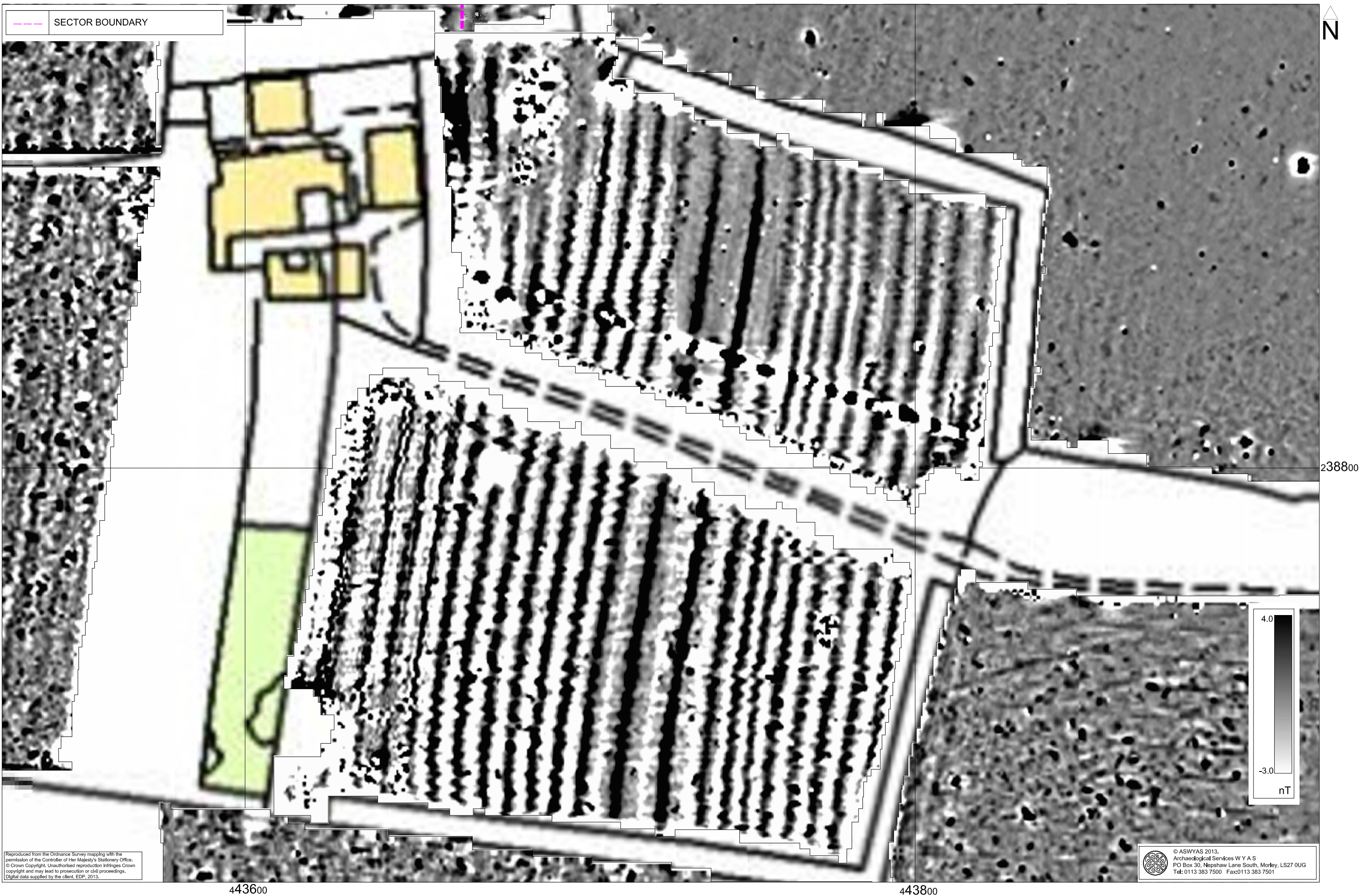
Fig. 26. Processed greyscale magnetometer data; Field 7 and Field 8 (1:1000 @ A3)
