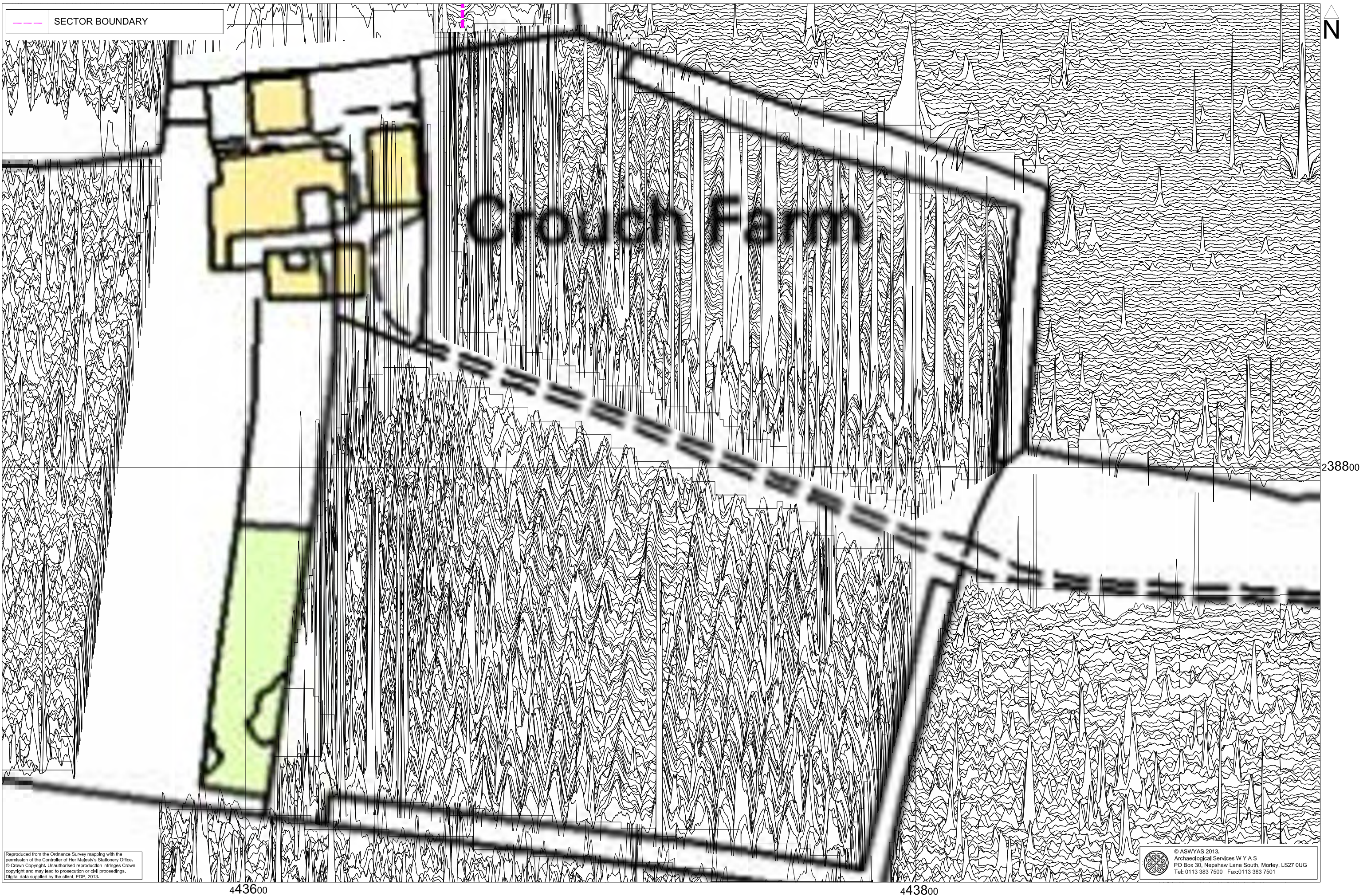
Fig. 27. XY trace plot of minimally processed magnetometer data; Field 7 and Field 8 (1:1000 @ A3)
