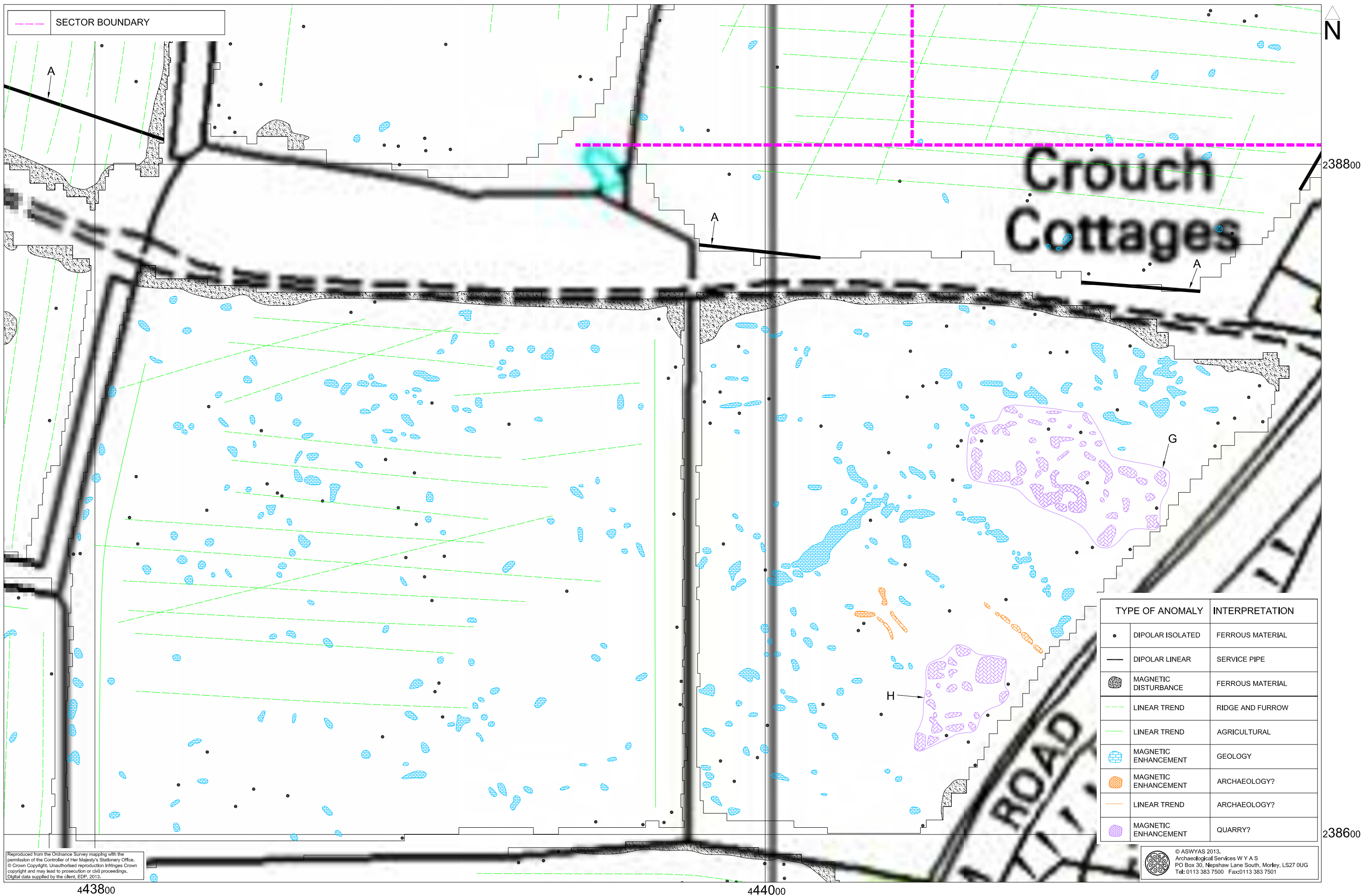
Fig. 16. Interpretation of magnetometer data; Field 4, Field 5 and Field 3, Sector 3 (1:1000 @ A3)
