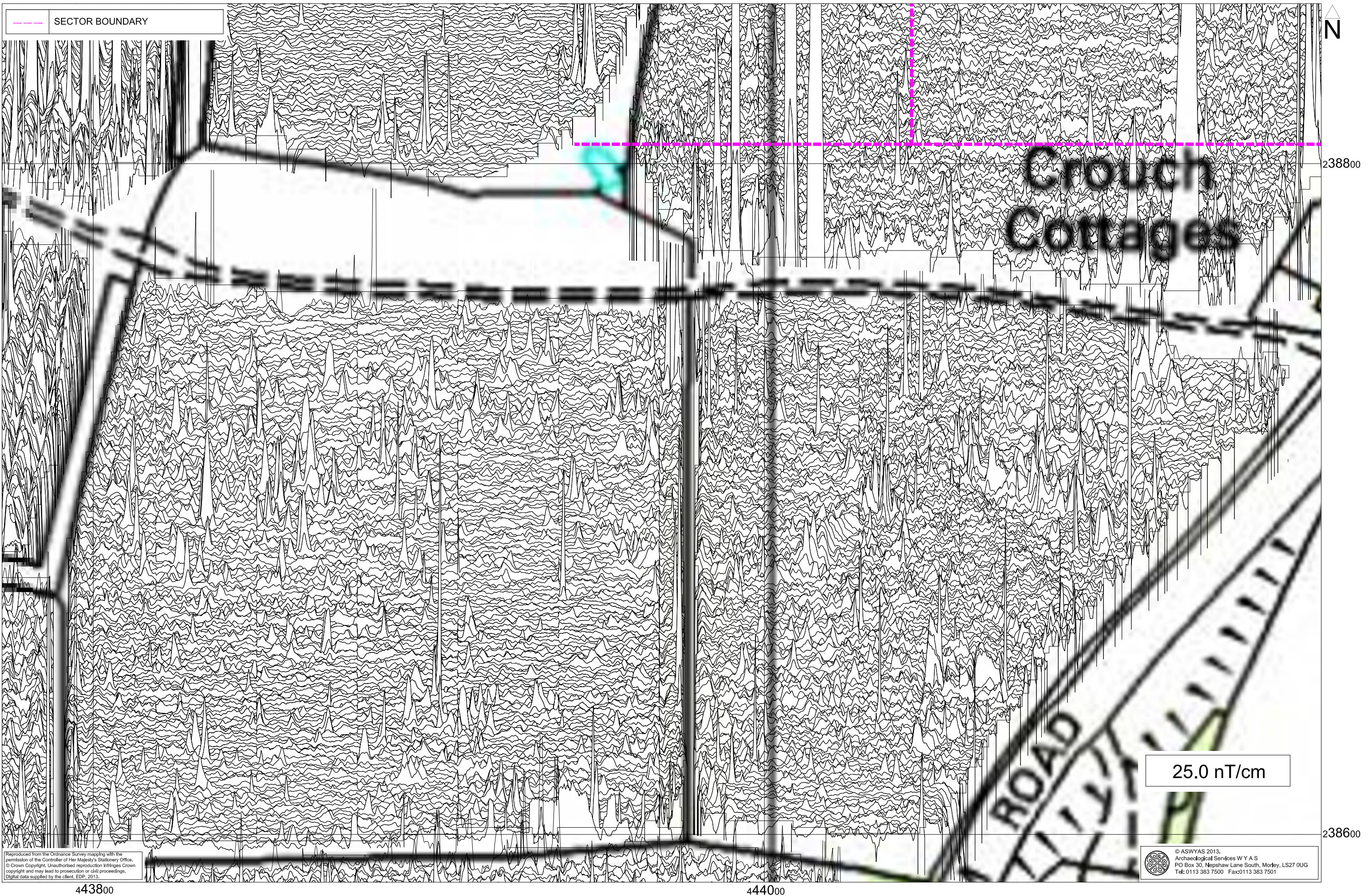
Fig. 15. XY trace plot of minimally processed magnetometer data; Field 4, Field 5 and Field 3, Sector 3 (1:1000 @ A3)
