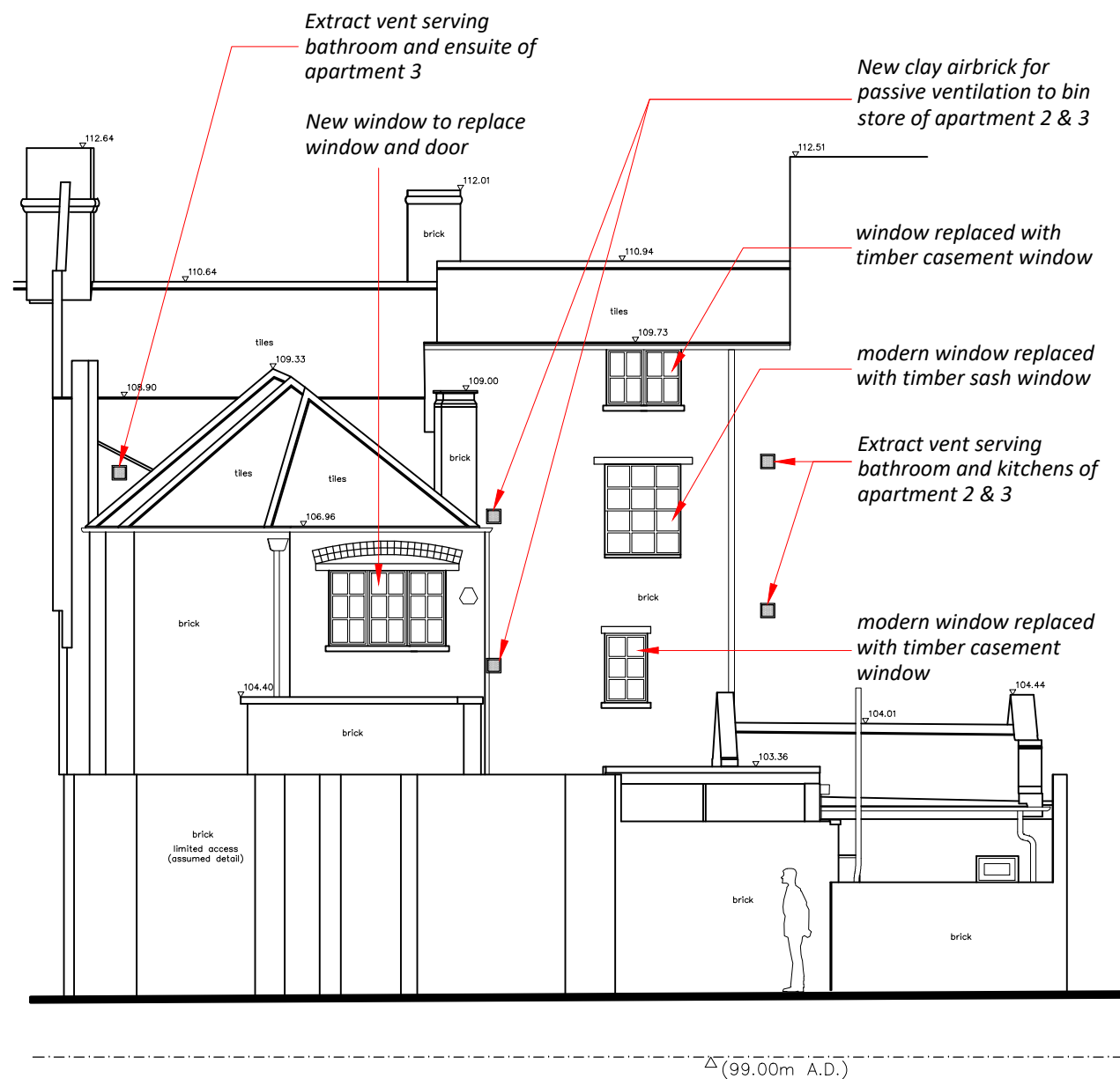
01 NORTH-WEST ELEVATION 1:100
