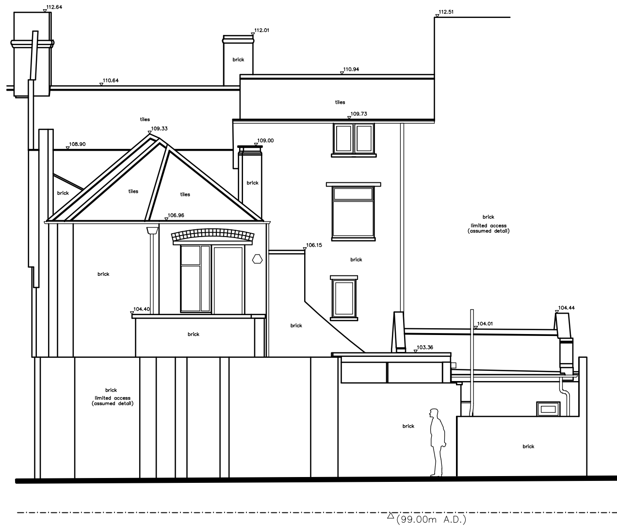
01 NORTH-WEST ELEVATION 1:100
