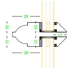
Glazing Bar to suit Heritage 7mm Slightline
