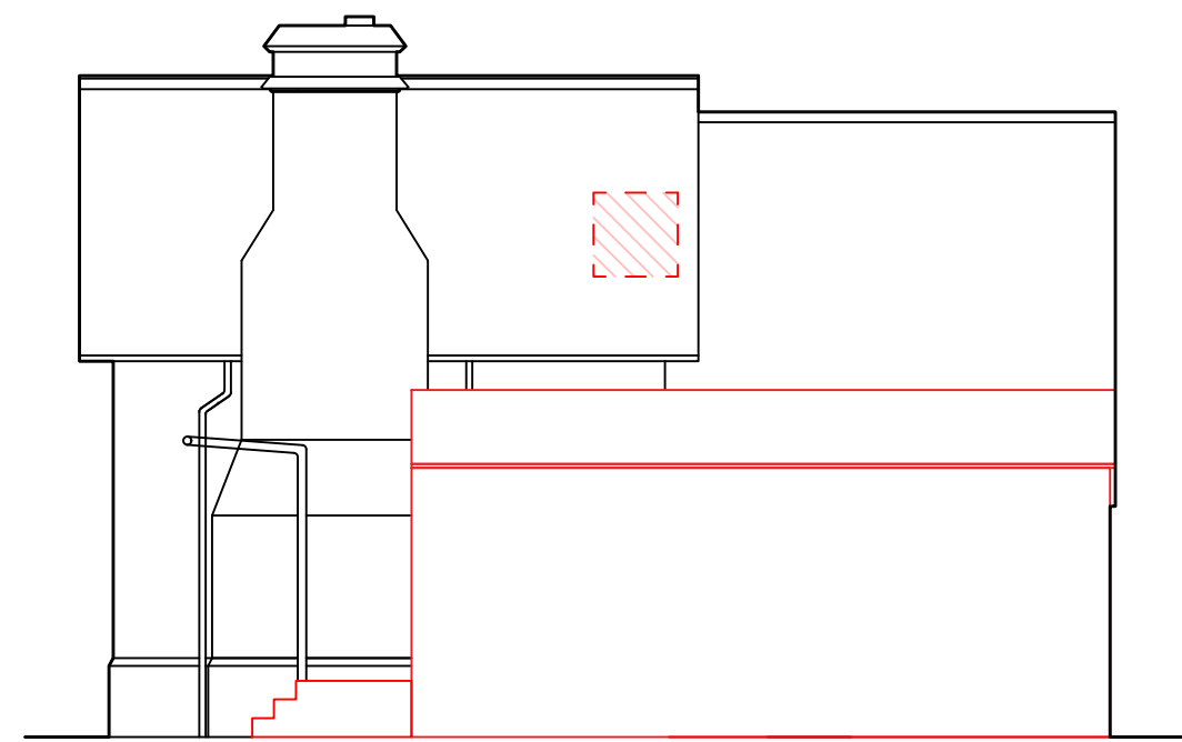
NORTH ELEVATION
