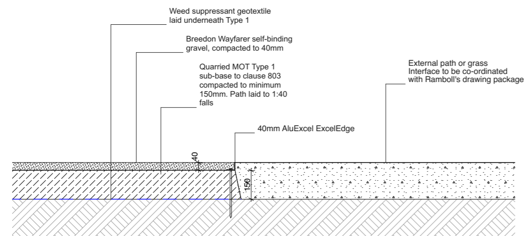
1 Self-binding gravel single path detail 1:20
