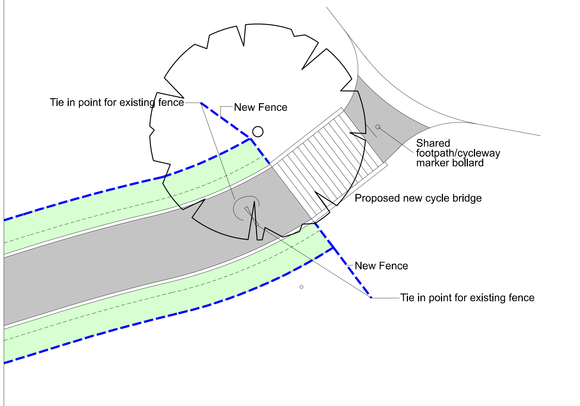
Indicative Proposed new cycle bridge 1.4m parapet 3m wide
