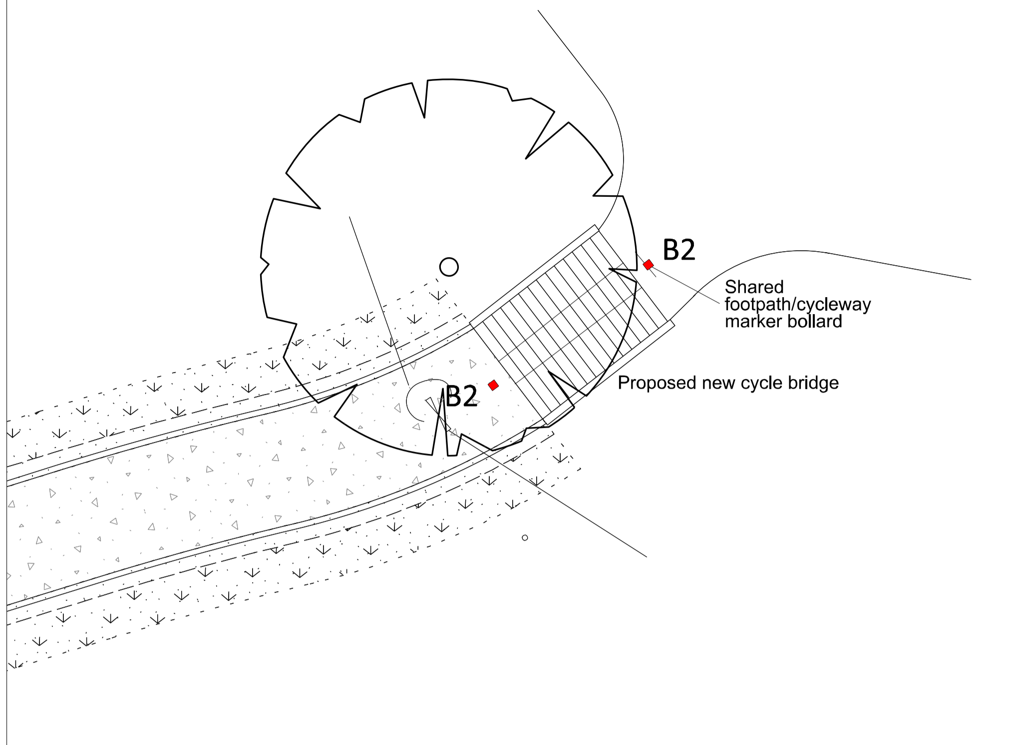
Indicative Proposed new cycle bridge 1.4m parapet 3m wide
