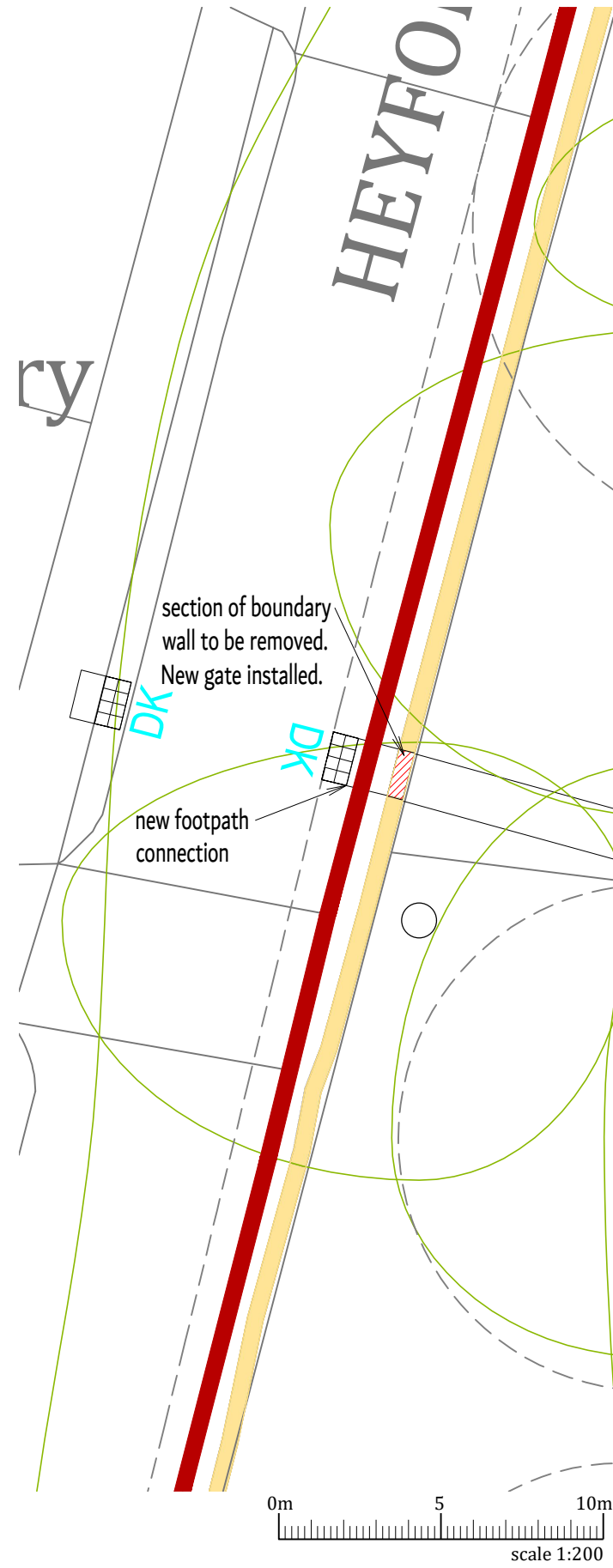
BOUNDARY WALL PLAN 1:200/ 1:1000 @ A3 KIR-PL04 LAND OFF HEYFORD ROAD KIRTLINGTON
