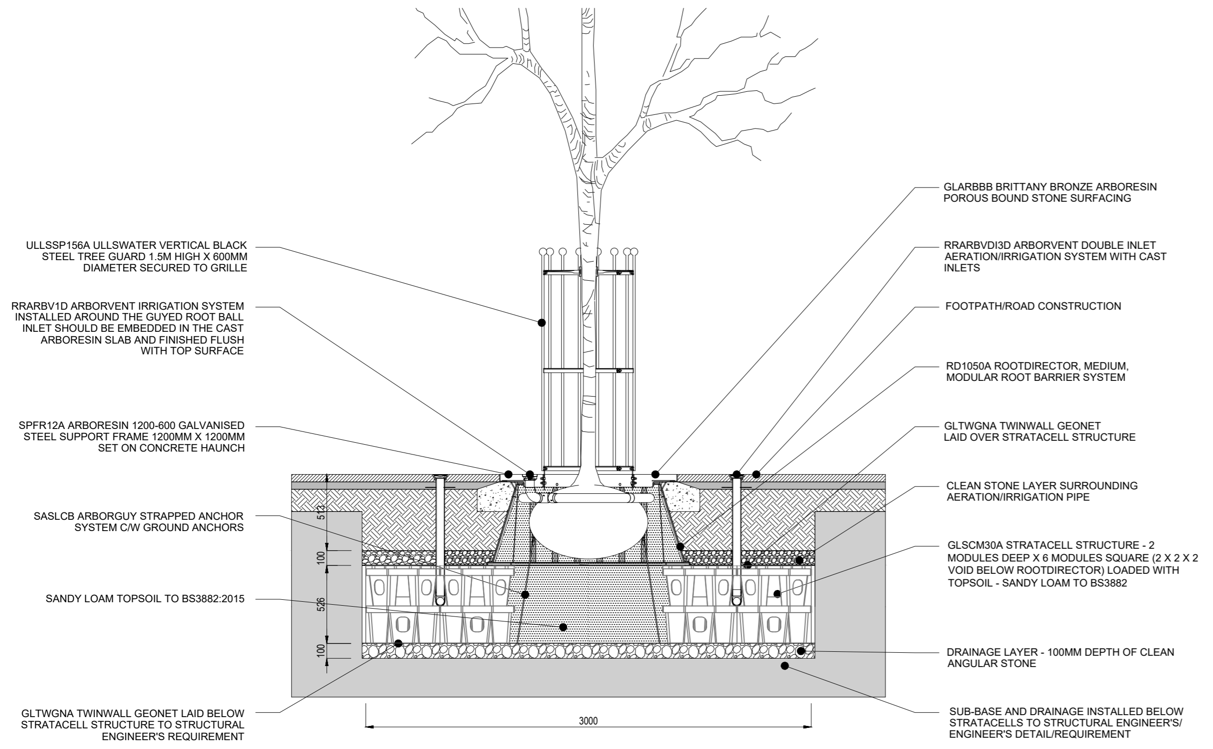
D) TREE PIT DETAIL (in hard paving)
