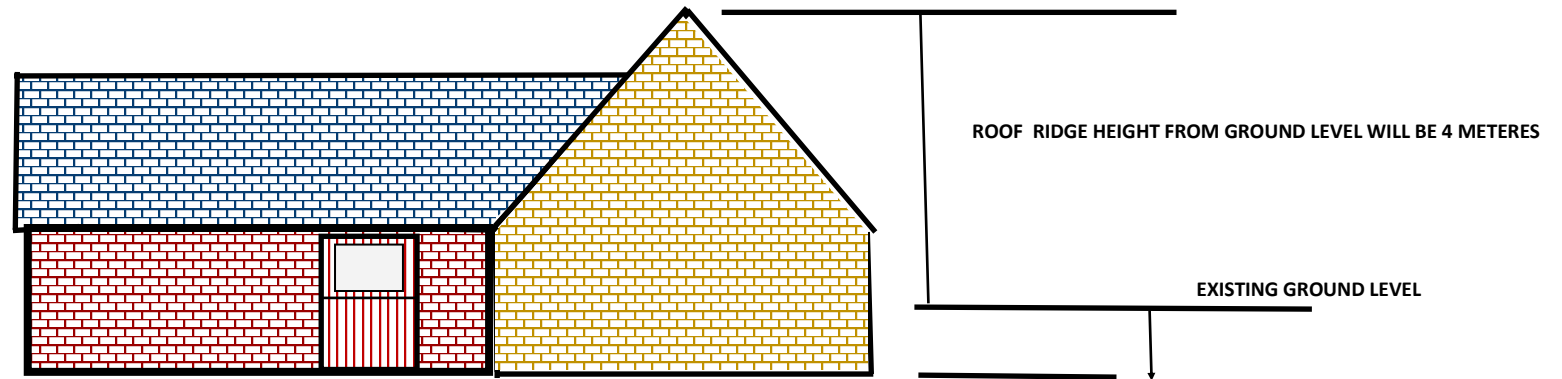
EAST ELEVATION
