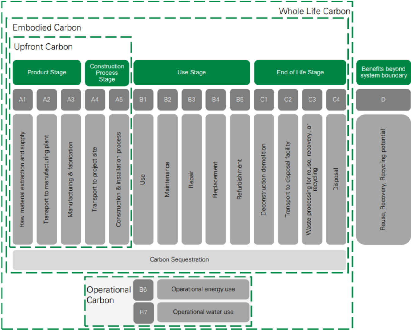
Figure 16.1 – Diagram showing the stages of the Life Cycle Assessment
