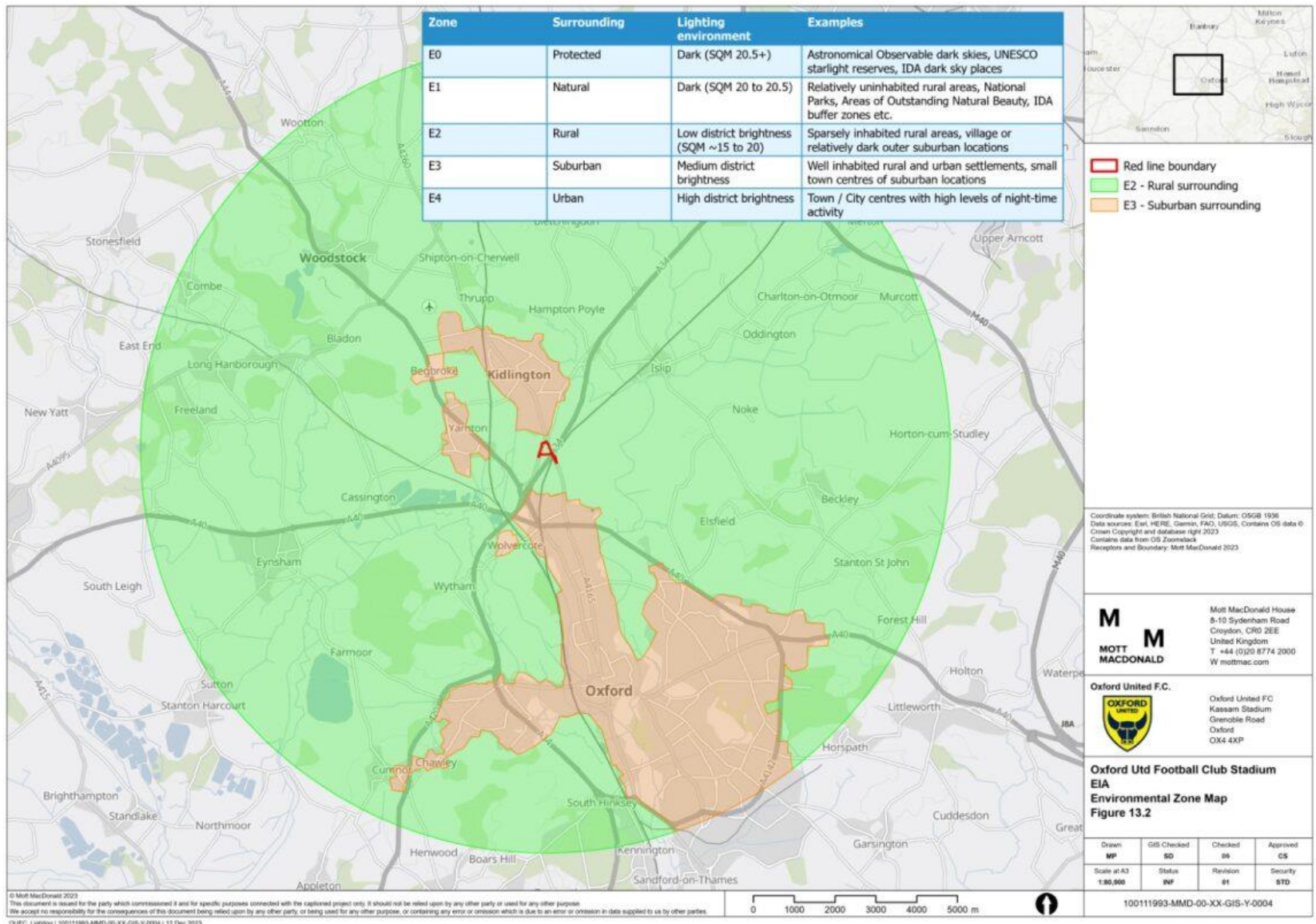
Figure 13.2 - Environmental Zones
