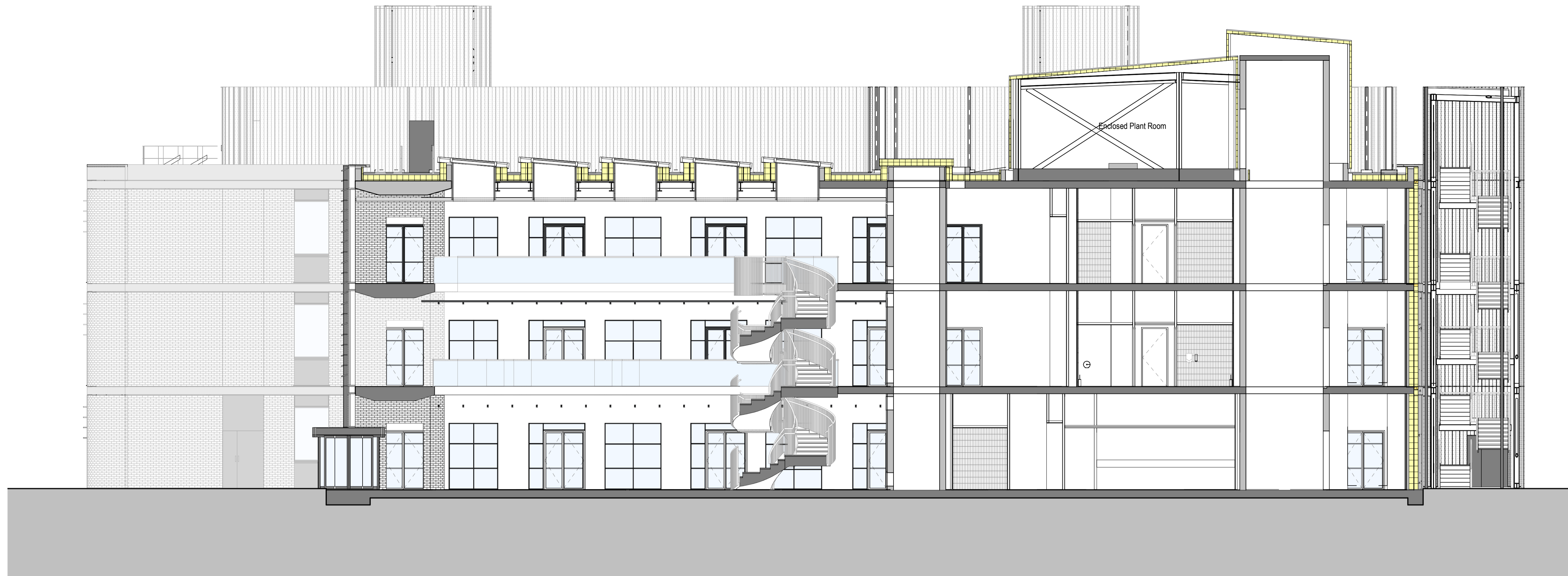
1 PLANNING - PROPOSED SECTION CC - COMMERCIAL BUILDING
