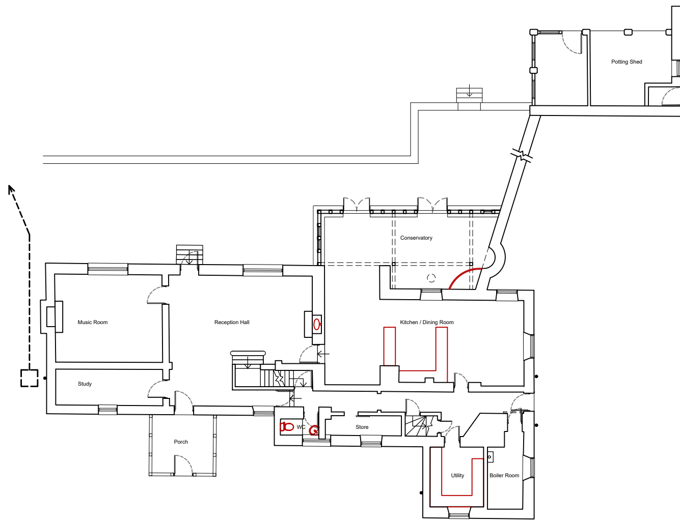
EXISTING GROUND FLOOR PLAN 1:200
