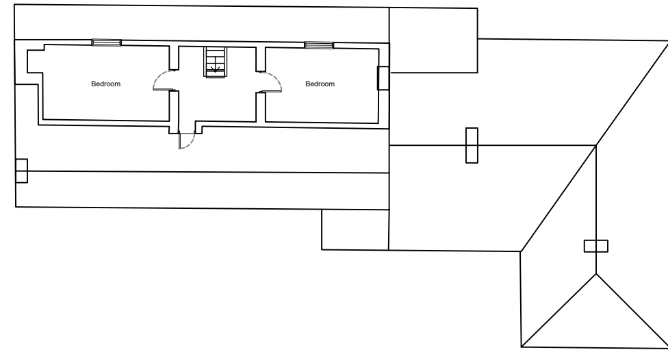
EXISTING SECOND FLOOR PLAN 1:200
