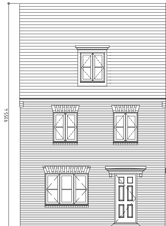
FRONT ELEVATION
